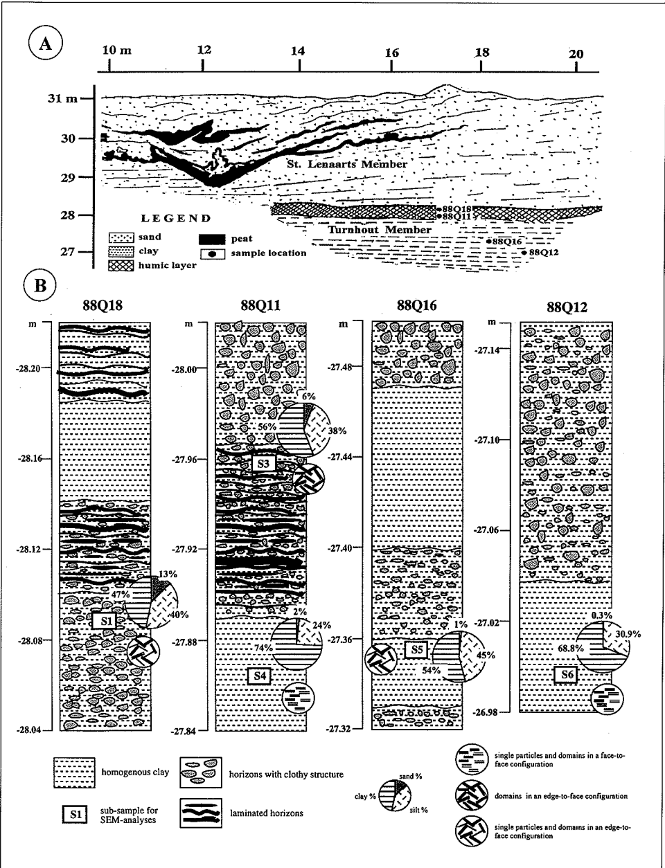
Fig. 2 — A - Geological section of the east-wall in the NOVA excavation, Beerse. B - Graphic representation of the radiographs from the Turnhout Member with indication of the observed clay-fabric types and sand-silt-clay ratios.
