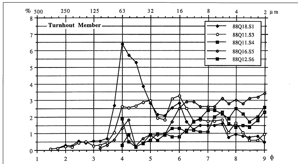
Fig. 4 — Grain-size spectra of samples from the Turnhout Member. Location of the samples is given in Figure 1.
