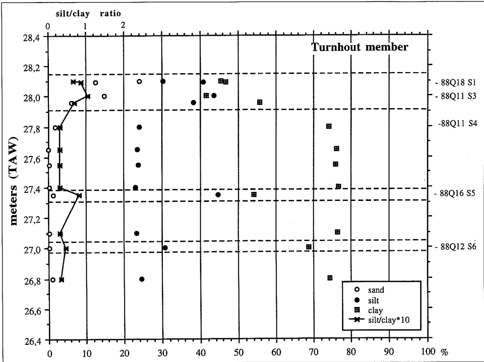
Fig. 3 — Distribution of sand, silt and clay in the clay-unit of the Turnhout Member
