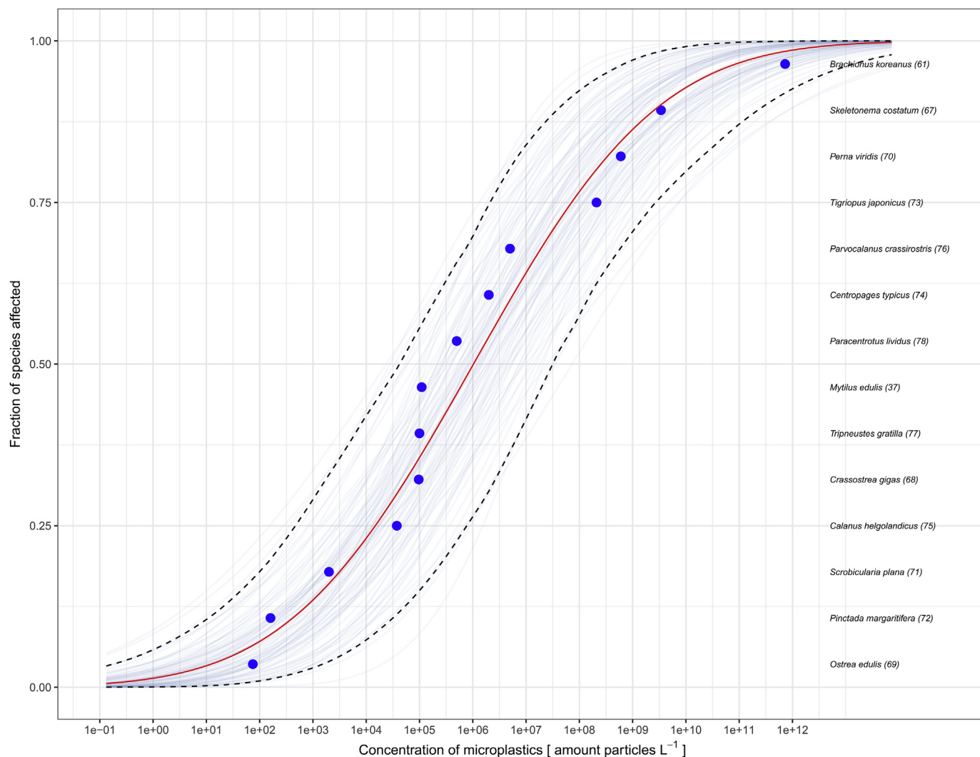
Fig. 2. Species sensitivity distribution (SSD) for buoyant microplastics (in particles L -1 ). Chronic no observed effect concentrations (NOEC) and chronic lowest observed effect concentrations (LOEC) were derived using standard procedures (Table 1). If several chronic NOEC or LOEC values for different toxicological endpoints were available for a single species, the lowest value was used. Note that a log-normal distribution is fitted and that the labels indicate the species that was exposed to microplastics. Detailed information on the effect data from literature, i.e. marine species exposed to microplastics, the size of the particles, the type of plastics used, and the endpoints used to assess the potential effects are available in Table 1 and supportive information. Blue dots are the NOECs of each species. The actual species sensitivity distribution is depicted in red and is surrounded by a confidence interval (black dotted lines) derived using 1000 random parameter iterations (grey lines) of the lognormal distribution. Numbers between brackets refer to the reference list. (For interpretation of the references to colour in this figure legend, the reader is referred to the Web version of this article.)
