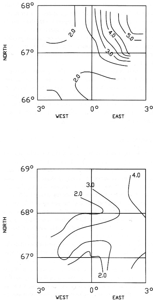
Figure 3. Temperature distribution at 300 m depth in the study areas in April 1995 (upper) and April 1996 (lower). Contours are in °C.
