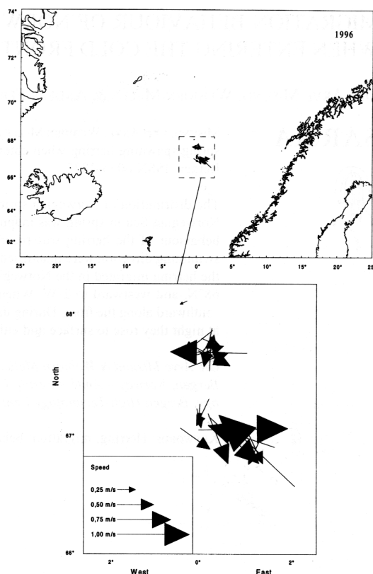
Figure 2. Study area (upper) and migration vectors (lower) of herring schools tracked for 4.2-121.8 min in April 1996.
