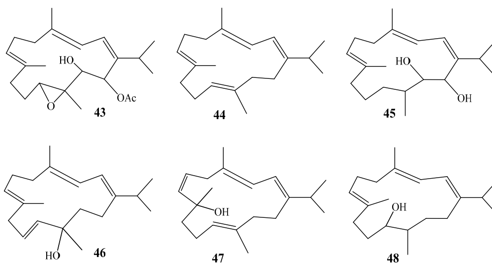
Figure 7. Chemical structures of compounds 43–48.
