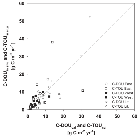
Fig. 9. Comparison of the in situ measured diffusive and total oxygen uptake rates and calculated fluxes from the two fitted regressions (Eqs. (4) and (5)).
