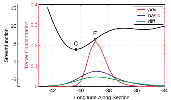
Fig. 17. Tracer concentration along the \sim A1E line after 2 yr, for the three model experiments, shown in relation to the streamfunction (black line) along the \sim A1E line. The edge and center of the Irminger gyre, discussed in Figs. 15 and 16, are denoted by the points E and C, respectively.
