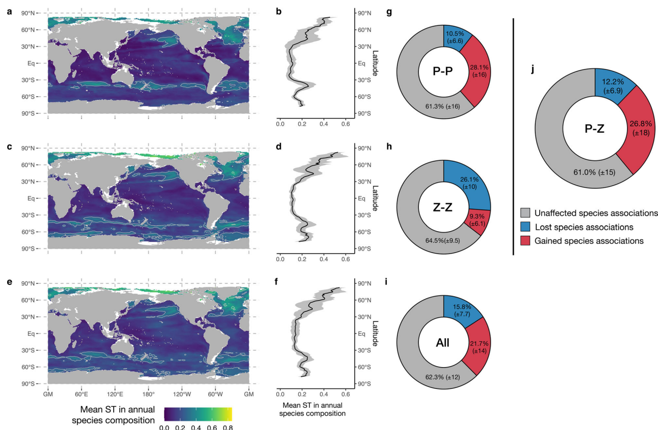
Fig. 3 Global patterns of species turnover (ST, true turnover component of Jaccard's dissimilarity index) and changes in species associations between 2012–2031 and 2081–2100. a Map of annual mean ST of phytoplankton species and its zonal average ( b ). c and d same as a and b but for zooplankton. e and f same as a and b but for all plankton. g Changes in phytoplankton species associations with the color indicating the percentage of species associations that are lost (blue), gained (red), or that remain constant (gray). h same as g but for zooplankton. i same as g but for all plankton. j as g but for the associations between phyto- and zooplankton species. The median (±IQR) relative contribution (%) of the three types of species associations to the total number of species associations identified as significant in the contemporary and future ocean are given in g , h , i , and j . The pale contour lines in a , c , and d indicate the isopleths of 25% mean ST. The gray contours in b , d , and f illustrate the standard deviation (std) associated with the zonal average displayed by the bold line. Total sample size is N = 35,023 grid cells.
