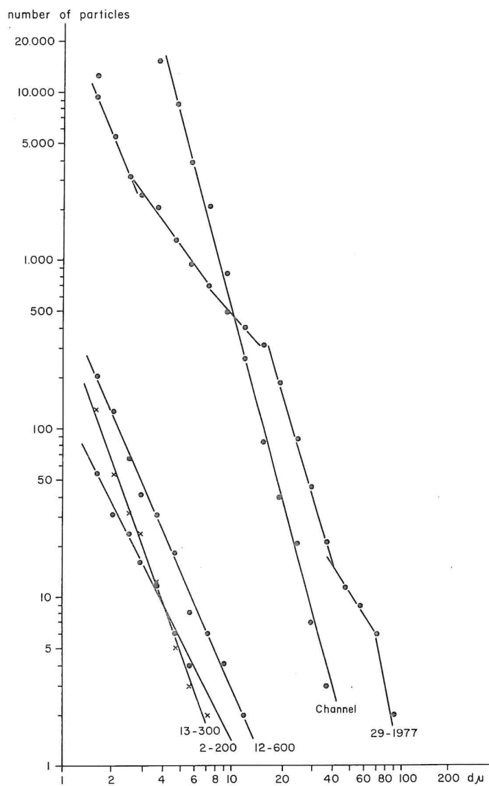
Fig. 7. Relation between \log d (particle diameter) and \log N (particle number).
