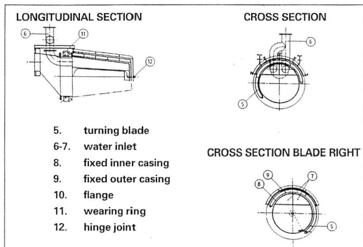
Figure 1. The scoop-head (general lay-out).
