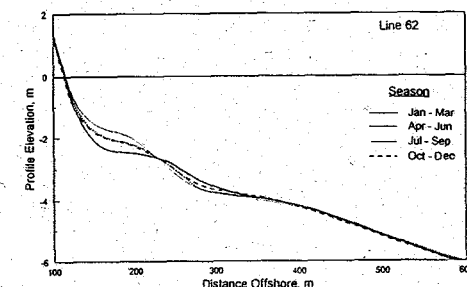
Fig. 11. Average seasonal profiles: Jan-Mar. Apr-Jun. Jul-Sep. and Oct-Dec. Line 62 (only portion with main change shown).
