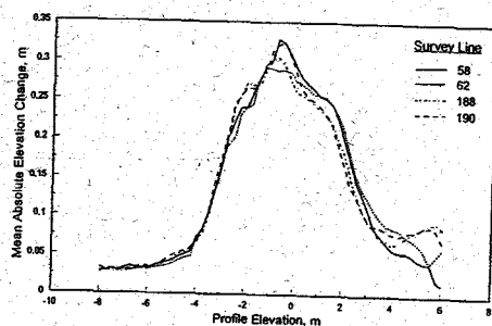
Fig. 8. Average absolute elevation change across shore, Lines 58, 62, 188, and 190.
