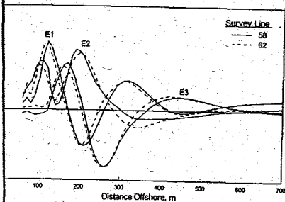
Fig. 5. First three eigenvectors for Lines 58 and 62.
