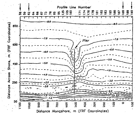
Fig. 2. Locations of survey lines relative to the FRF research pier and bathymetry on 9 September 1988 (depths in meters relative to NGVD) (after Leffler et al., 1990).
