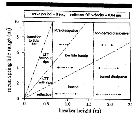
Figure 6. Location of modal beach types based on threshold values of breaker height and mean spring tide range for a beach with wave period T = 8 sec and the fall velocity w = 0.04 m/sec ( D_{50} = 0.3 mm). The boundaries between beach types, as indicated by the dotted lines, will shift in response to changes in T and w . The arrows in the diagram indicate the direction and relative, not absolute, rate of response to temporal changes in wave height. Beach response decreases with increasing tide range and decreasing wave height, and response to rising waves is faster than to falling waves (WRIGHT et al. , 1985).
