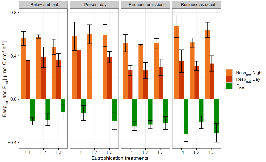
Figure 6: Net respiration rates ( \text{Resp}_{\text{net}} ) and net photosynthetic rates ( \text{P}_{\text{net}} ) of the holobiont (sponge + symbionts) during the day and night \pm SEM for each p\text{CO}_2 and eutrophication scenario.
