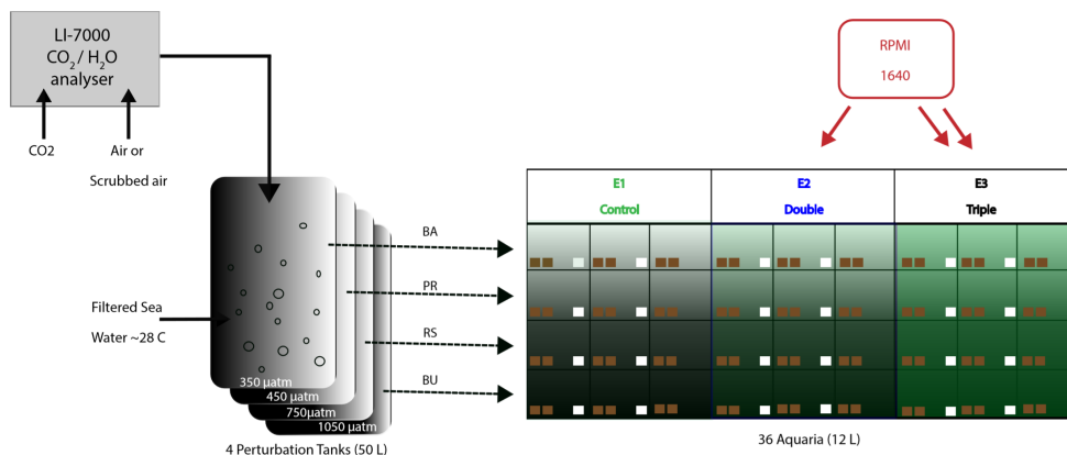
Figure 1: Experimental setup consisting of four large barrels in which the p\text{CO}_2 (4 levels) is manipulated and controlled through a central CO 2 sensor. From every barrel water is pumped into 9 aquaria (12 L each). Of these 9 two groups of 3 aquaria were supplied with additional dissolved organic carbon (E1: green, E2: blue, E3: black) using peristaltic pumps. Pumps ran at different speed between E2 and E3 to deliver different concentration of RPMI. Each of the 36 aquaria contained 2 sponge bearing coral cores (brown squares) and 24 aquaria contained control cores (white squares).
