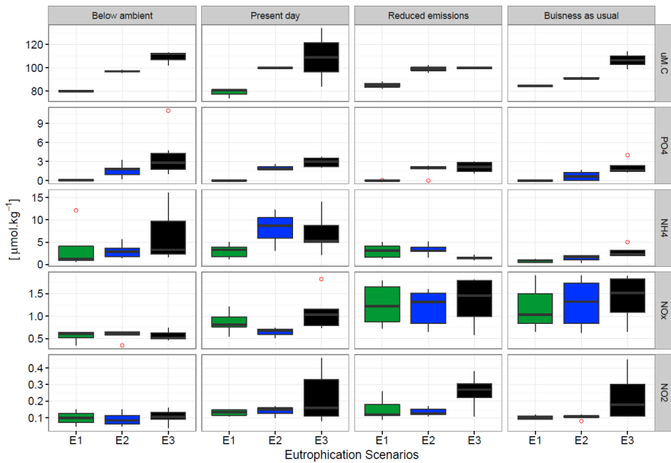
Figure S 1: Boxplot of initial nutrient and dissolved organic carbon (uM.C) concentrations for each p\text{CO}_2 scenario (top) and eutrophication treatments (E1, E2, E3) (n=59).
