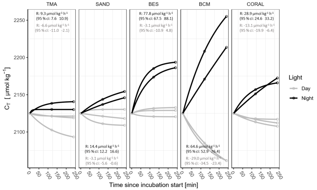
Figure 6: Results of the model employed (equation 3) to infer every C_T^{resp} input rates ( \mu\text{mol kg}^{-1} \text{ h}^{-1} ) from observations for each substrate recorded during the day (grey) and at night (black). Circles represent discrete C_T^{resp} values measured at T_0 , T_2 and T_4 . Average rates and respective 95% confidence interval are depicted for each substrate and light.
