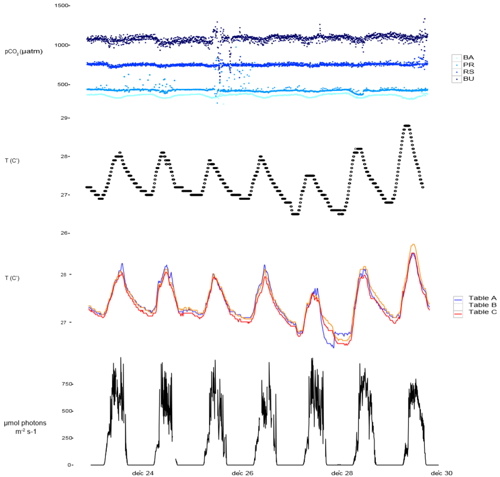
Figure 2: Temporal variability from December 23 to December 30 2015 of continuously monitored pCO 2 (a), temperature monitored in the barrels used for setting the pCO 2 experiments (b), temperature measured directly in aquaria from table A.B and C (c) and light throughout the 1 week experiment.
