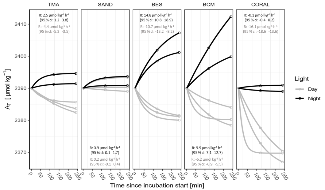
Figure 5: Results of the model employed (equation 3) to infer every A_T input rates ( \mu\text{mol kg}^{-1} \text{ h}^{-1} ) from observations for each substrate recorded during the day (grey) and at night (black). Circles represent discrete A_T values measured at T_0 , T_2 and T_4 . Average rates and respective 95% confidence interval are depicted for each substrate and light.
