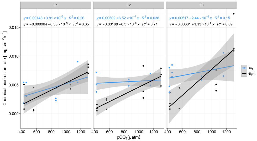
Figure 3: Chemical bioerosion rates in \text{mg cm}^{-2} \text{ h}^{-1} as a function of p\text{CO}_2 for day and night and each eutrophication treatment. Linear regressions illustrate positive correlation between p\text{CO}_2 and dissolution rates. Slopes are significantly different between day (blue) and night (black) but not between eutrophication scenarios (E1-E3). Alkalinity titrations for incubations in Present scenario (PD) and E2 treatment during the day were of questionable quality due to equipment failure and therefore not represented here (n=59).
