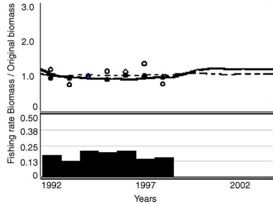
Fig. 3. Fitting independent data on relative biomass as CPUE (dots) to Ecosim-simulated biomass (lines) of target species in La Paz Bay, Mexico. Shaded area represents the historic fishing pattern. Black dots and dashed line represent snappers; open dots and lines, groupers.
