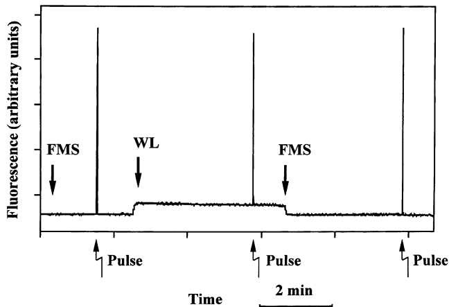
Fig. 1. Changes in fluorescence signal measured in F. vesiculosus exposed to low actinic light (ca. 20 \mu\text{mol m}^{-2} \text{s}^{-1} ) of different quality. Arrows indicate which actinic light is on: WL, cold white light provided by the Intralux 4000-1; FMS, red-enriched light provided by the FMS.
