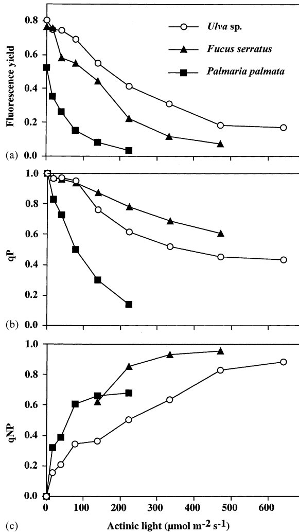
Fig. 4. Changes in fluorescence parameters and quenching coefficient, as a function of actinic light intensity, for: Ulva sp. , P. palmata , and F. serratus : (a) F_v/F_m (after dark adaptation) and PSII (actinic light on); (b) photochemical quenching qP; (c) nonphotochemical quenching qNP. For qNP calculation, during exposure to actinic light higher than ca. 200 \mu\text{mol m}^{-2} \text{s}^{-1} , F_s was often lower than F_0 in F. serratus . In these conditions, quenching analyses were made possible by the measure of F'_0 , fluorescence emission obtained after exposition to far-red light (PSIIR function), i.e. corresponding to the fluorescence signal in a light-adapted state with all PSII reaction centres open. In an alternative way, F'_0 can be estimated according to Oxborough and Baker (1997).
