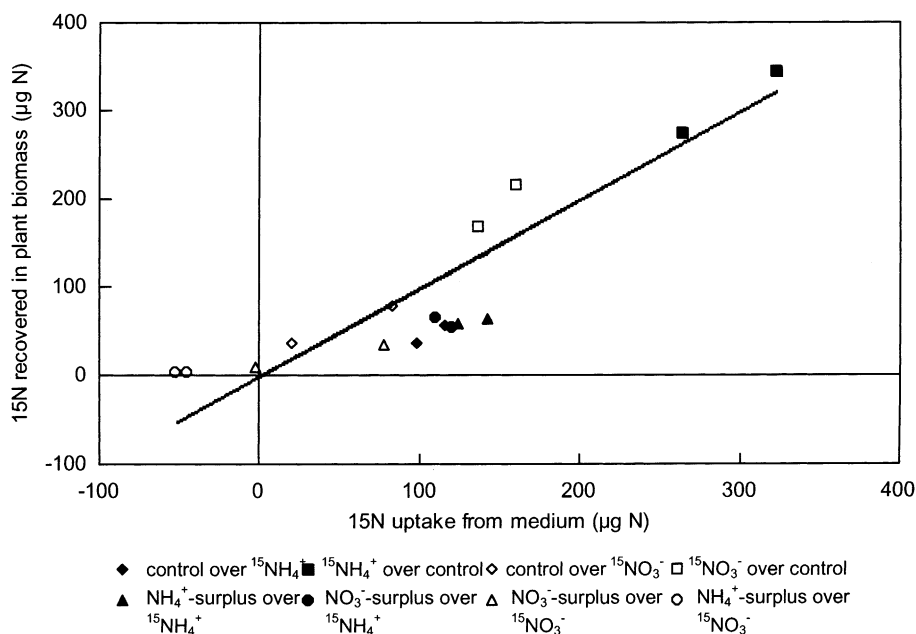
Fig. 4. Comparison of amounts of ^{15}\text{N} recovered from above-ground and below-ground plant material with calculated uptake from the incubation medium. The solid line represents the 1:1 slope.
