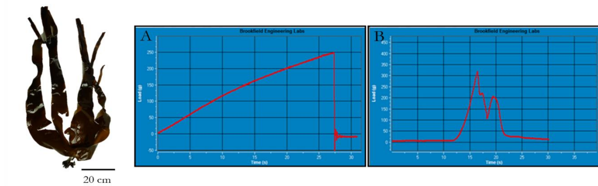
Figure 1-12. Exemplary graphs of (A) ultimate tensile strength (UTS) and (B) ultimate piercing load (UPL) during texture analysis (analyzer: CT3, Brookfield Engineering, USA) of a Laminaria digitata frond.
