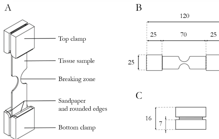
Figure 5-3. (A) Sketch of set up to analyse UTS. The tissue sample is fixated between top and bottom clamp (attached to the texture analyser). The clamps have rounded edges to avoid damage and a layer of sandpaper prevents the sample from slipping during UTS analysis. (B) Front view and metric dimensions (mm) of the set up with clamps. (C) Top view and metric dimensions (mm) of a clamp (round edges not illustrated).
