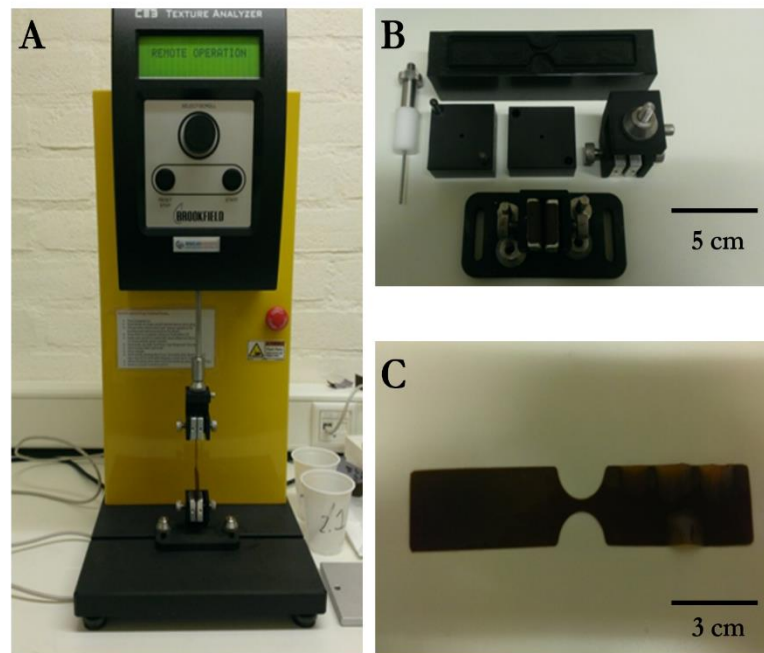
Figure 1-7. A) Front view on fittings of the texture analyser (CT3, Brookfield Engineering, USA) with attached seaweed sample, B) customized clamps, sample attachments and sample stamp for toughness measurements on seaweed (bottom to top) and C) punched out sample of a Laminaria digitata frond, ready for toughness analysis.
