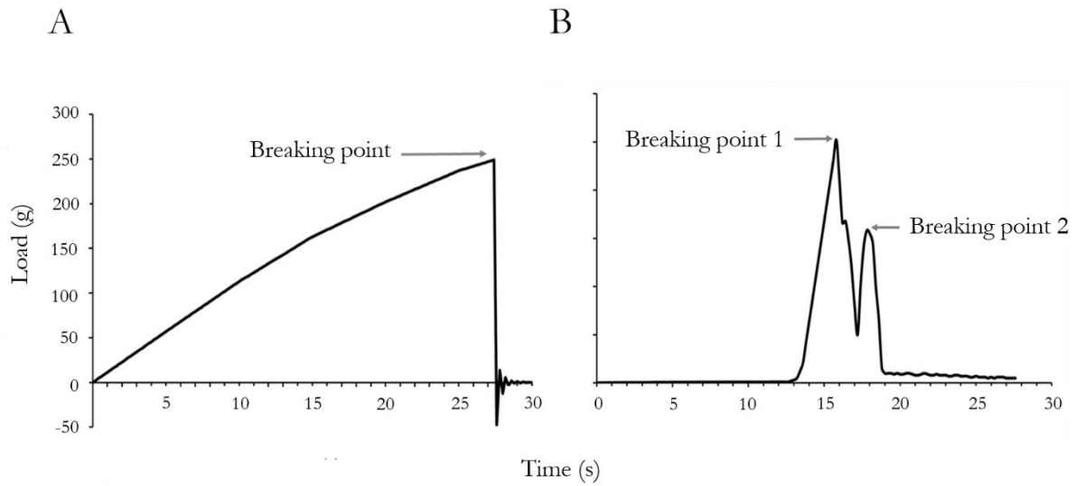
Figure 5-5. Typical graph of tension (A) and compression (B) measurements during texture analysis of L. digitata samples. (A) The breaking point indicates the rupture of the sample, referred to the ultimate tensile strength (UTS) of the tissue. (B) Breaking point 1 indicates the rupture of the external cell wall by punctuation needle, the ultimate piercing load (UPL). Breaking point 2 represents the internally initiated rupture of the cell wall on the opposite side.
