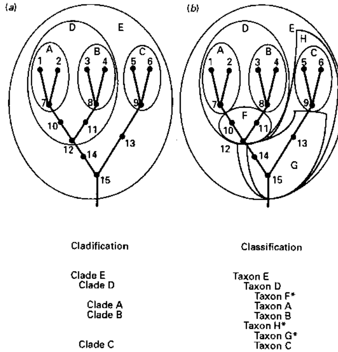
Fig. 2. Contrast between (a) cladification and (b) classification. From the same phylogenetic tree with holophyletic recent species 1 to 6 and paraphyletic ancestral species 7 to 15 one can produce either a list of nested clades or a comprehensive classification. In the classification taxon D is comprehensively subdivided into three taxa of lower and equal rank (A, B, F); A and B are holophyletic and F is paraphyletic. In the cladification, clade D is subdivided into two clades A and B with the same composition as the holophyletic taxa A and B plus a residue including species 10 to 12 which is not placed in any subgroup of clade D. The cladification is not a comprehensive classification of clade D, because this paraphyletic residue comprising species 10 to 12 is not listed under clade D even though it is part of that clade. The size of this paraphyletic residue could be reduced in an alternative cladification by moving the boundaries of clades A and B from just below species 7 and 8 to just above species 12; but as species 12 is ancestral to both clades A and B, it cannot be included in either. No clade can be comprehensively subdivided into subclades. A cladification can never be a comprehensive classification since it omits the paraphyletic residues which a comprehensive classification must include (taxa F, G and H in this case). The cladification on the left is congruent with the classification on the right. When comprehensively subdivided into taxa of equal rank, it is logically inescapable that every monophyletic taxon (whether holophyletic or paraphyletic) must include at least one paraphyletic taxon. A cladification is a most useful step towards a phylogenetic classification but it does not constitute one in its own right. If paraphyletic taxa are explicitly identified in a phylogenetic classification one can reconstruct the cladification on which it is based by deleting them. But one cannot move from a phylogenetic tree to a classification without exercising taxonomic judgement, which is necessary both in deciding which clades should be treated as taxa and whether the paraphyletic residue should be treated as a single taxon or subdivided. Judgement is likewise needed about the appropriate rank for each taxon.
