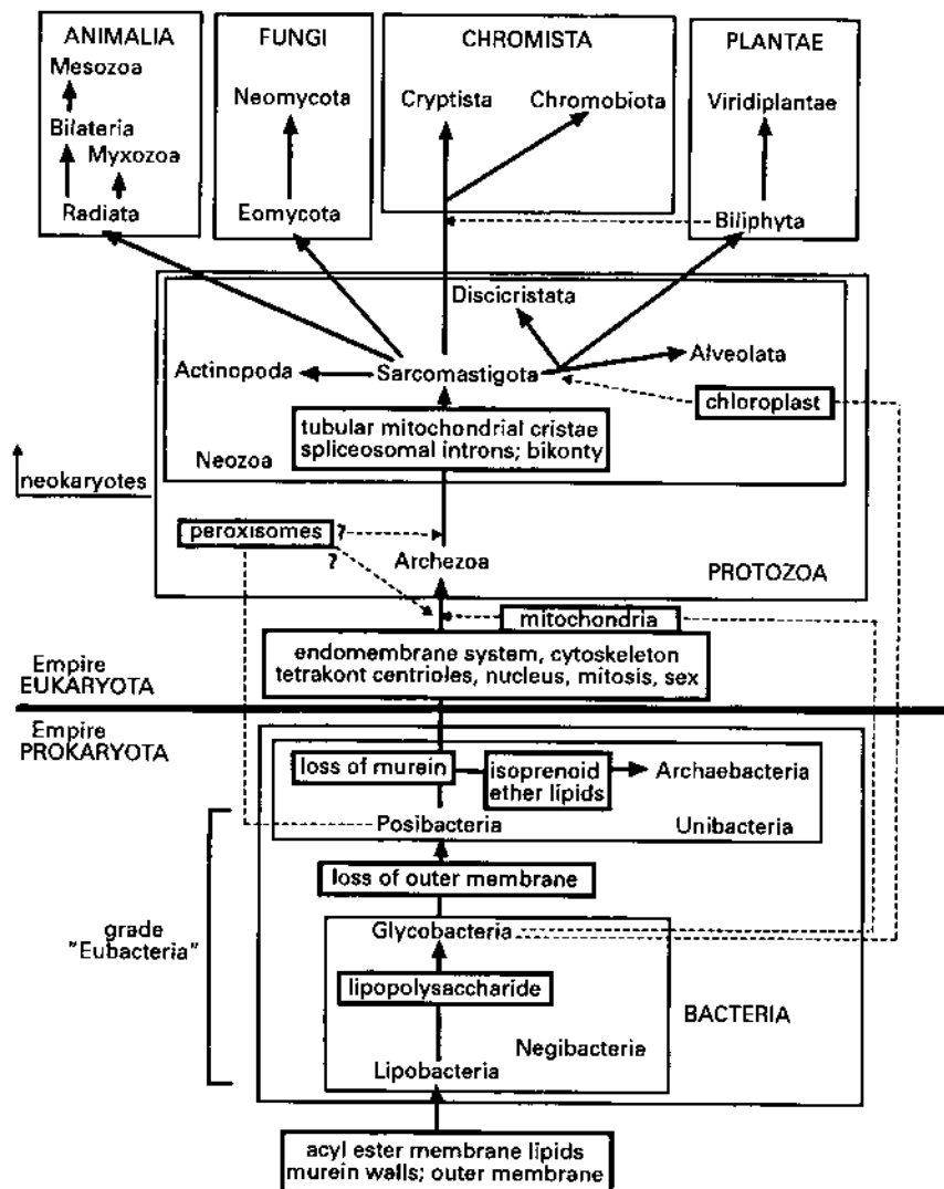
Fig. 1. Postulated phylogenetic relationships between the six kingdoms (upper case) and their subkingdoms. Infrakingdoms are also shown for the two basal paraphyletic kingdoms, as are some key innovations (within heavy boxes). The four major symbiogenetic events in the history of life are shown with dashed arrows: (1) the symbiogenetic origin of mitochondria from an \alpha -proteobacterium, (2) the probable origin of peroxisomes from a posibacterium (Cavalier-Smith, 1990), (3) the monophyletic origin of chloroplasts from a cyanobacterium, and (4) the origin of the ancestral chromist as a eukaryote-eukaryote chimaera between a rhodellophote red algal endosymbiont and a biciliated protist host; whether the host was a protozoan, as assumed here, or a very early plant is unclear. For clarity infrakingdoms are not shown for the four higher holophyletic kingdoms, Animalia, Fungi, Plantae, and Chromista. The diagnoses of the taxa are given in Table 1 and their composition is summarized in Tables 2-7. Chloroplasts are assumed to have originated in the latest common ancestor of Plantae, Discicristata and the alveolate dinoflagellate protozoa (Cavalier-Smith, 1982), and the plastids of euglenoids and alveolates are assumed to have arisen divergently from this primary endosymbiosis. However, the alternative possibility that dinoflagellates and/or euglenoids obtained their chloroplasts secondarily by lateral transfer from a chromiote and green alga respectively, though considered distinctly less likely, cannot currently be excluded (Cavalier-Smith, 1995a); the source of the non-photosynthetic plastid of coccidiomorph Sporozoa is equally uncertain (McFadden & Waller, 1997). For simplicity a fifth important case of symbiogenesis is not shown: secondary symbiogenetic lateral transfers of green algal, possibly ulvophyte (Ishida et al. , 1998), chloroplasts into a cercozoan (sarcomastigote) host to create the algal class Chlorarachnea (e.g. Chlorarachnion ). The least certain features of the tree are the position of its root (some authors favour a root within the Unibacteria rather than the Negibacteria) and of the Discicristata (18S rRNA and EF 1- \alpha trees put them below the Sarcomastigota, whereas other proteins place them as shown).
