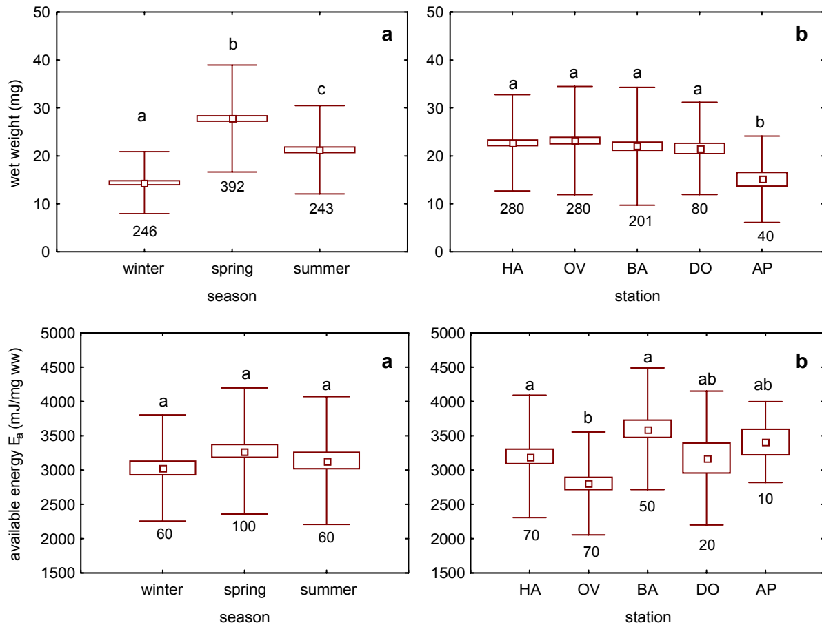
Figure 10.3. Seasonal (a) and spatial (b) patterns in wet weight (ww) and total energy content ( E_a ) of N. integer in the Scheldt estuary. Different letters indicate significant differences ( p < 0.05 ). Number below the whisker indicates the number of observations. Refer to Fig. 10.1 for sampling locations.
