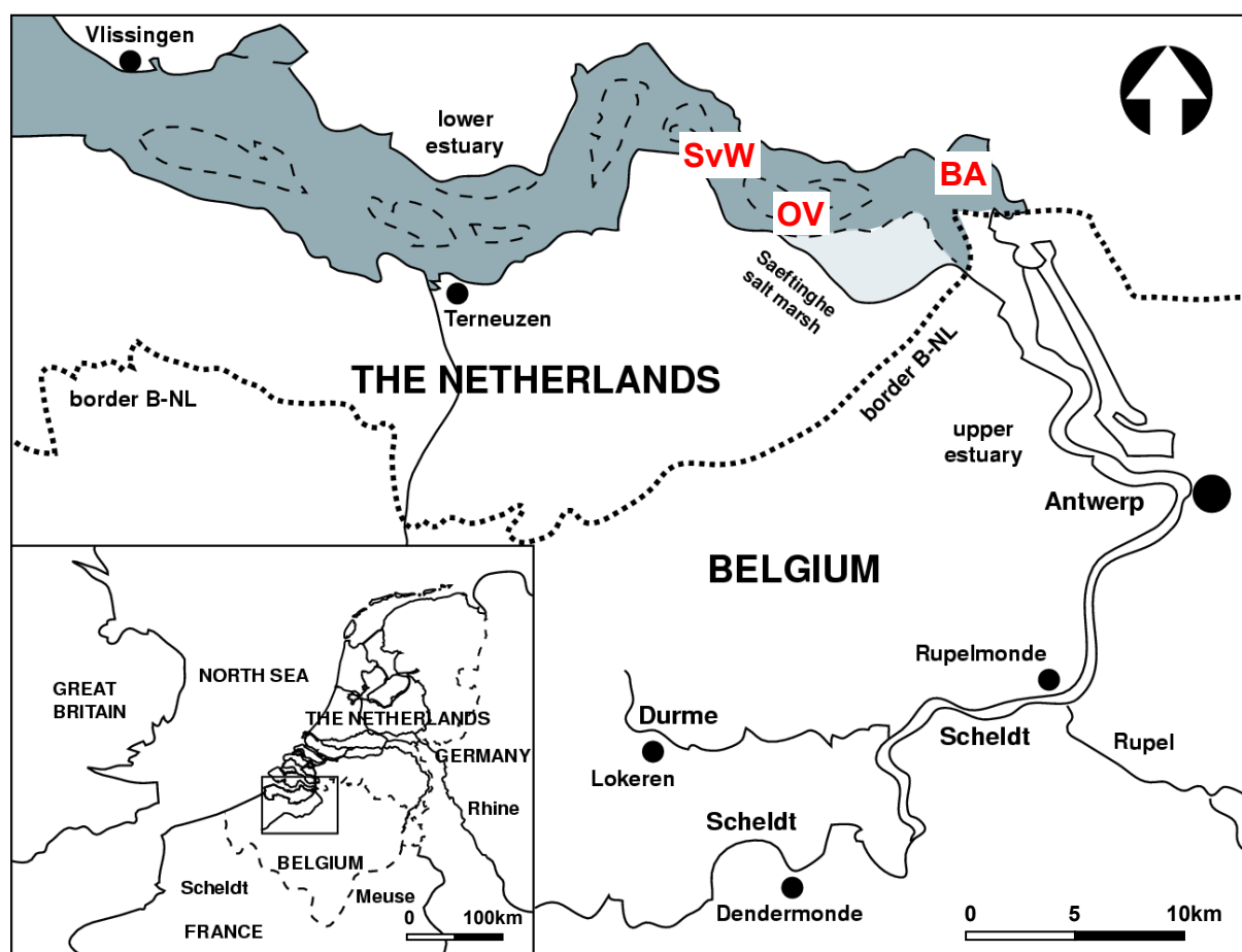
Figure 9.1. The Scheldt estuary, one of the largest and most polluted estuaries in Europe, was sampled for water, sediment and mysids at three sites (SvW, Schaar van Waarde; OV, Overloop van Valkenisse; BA, Bath) in november 2001, representative of the major distribution area of the estuarine mysid N. integer .
