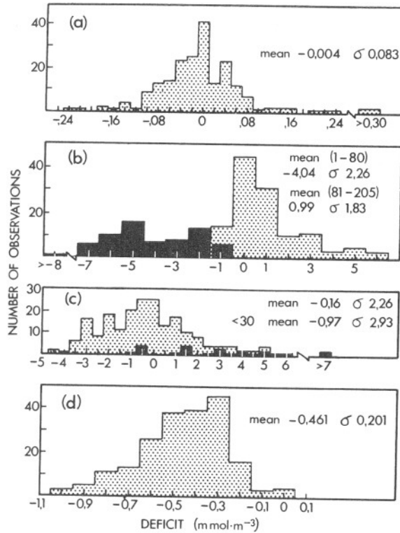
Fig. 4: Distribution of deficits from Cruise 067, shaded portions denoting nitrate samples 1-80 and silicate concentrations (measured at sea) greater than 30 \text{ mmol}\cdot\text{m}^{-3} respectively — (a) nitrite, (b) nitrate, (c) silicate, (d) phosphate
