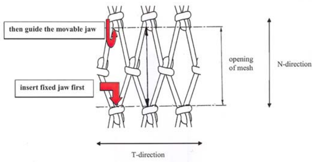
Figure 1. Insertion of the gauge.
