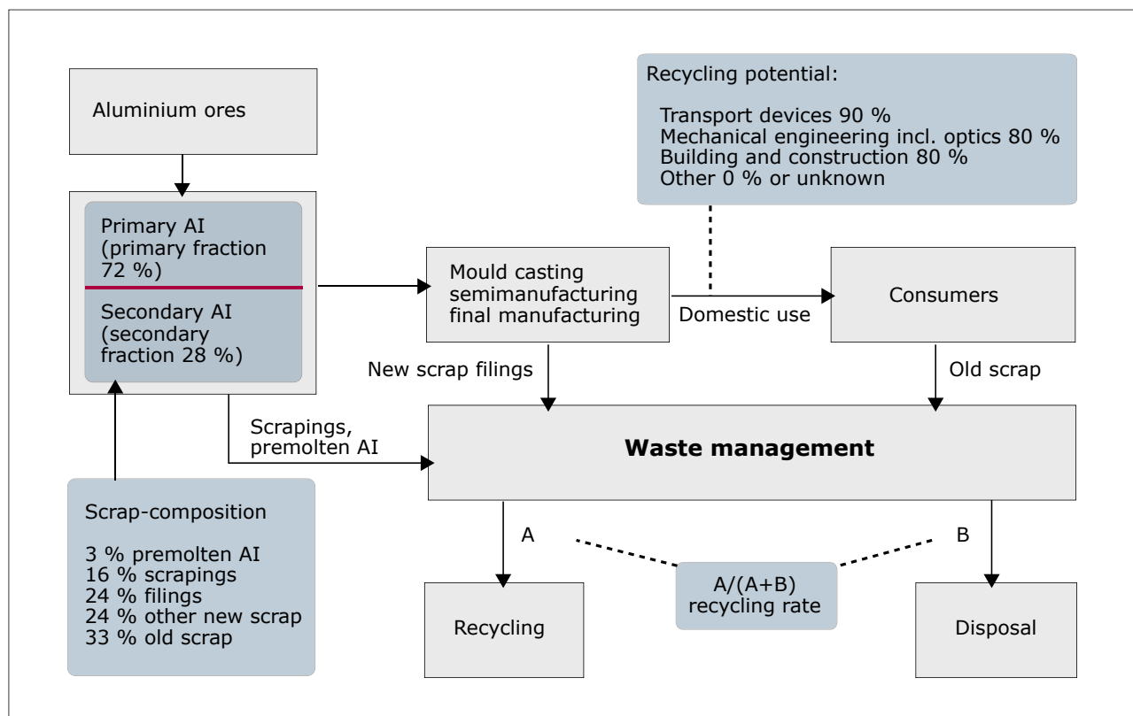
Figure 3.16 Recycling flows of aluminium
