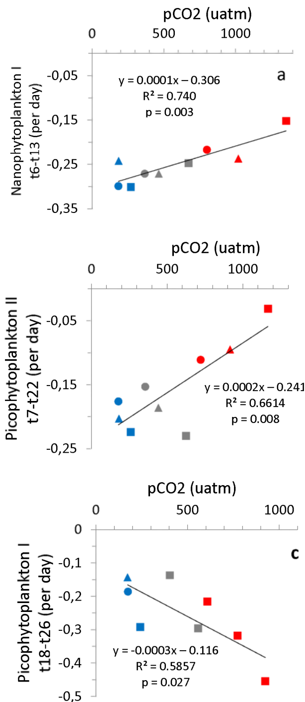
Fig. 5. Specific growth rates determined from the net phytoplankton abundances versus p\text{CO}_2 . Nanophytoplankton I from t6 – t13 (a), picophytoplankton II from t7 to t22 (b), and picophytoplankton I from t18 – t26 (c). A negative growth rate indicates cell loss. The \text{CO}_2 concentrations plotted were the averages for the specific time periods indicated. For color and symbol coding, see Fig. 1. Linear regression statistics provided in plots.
