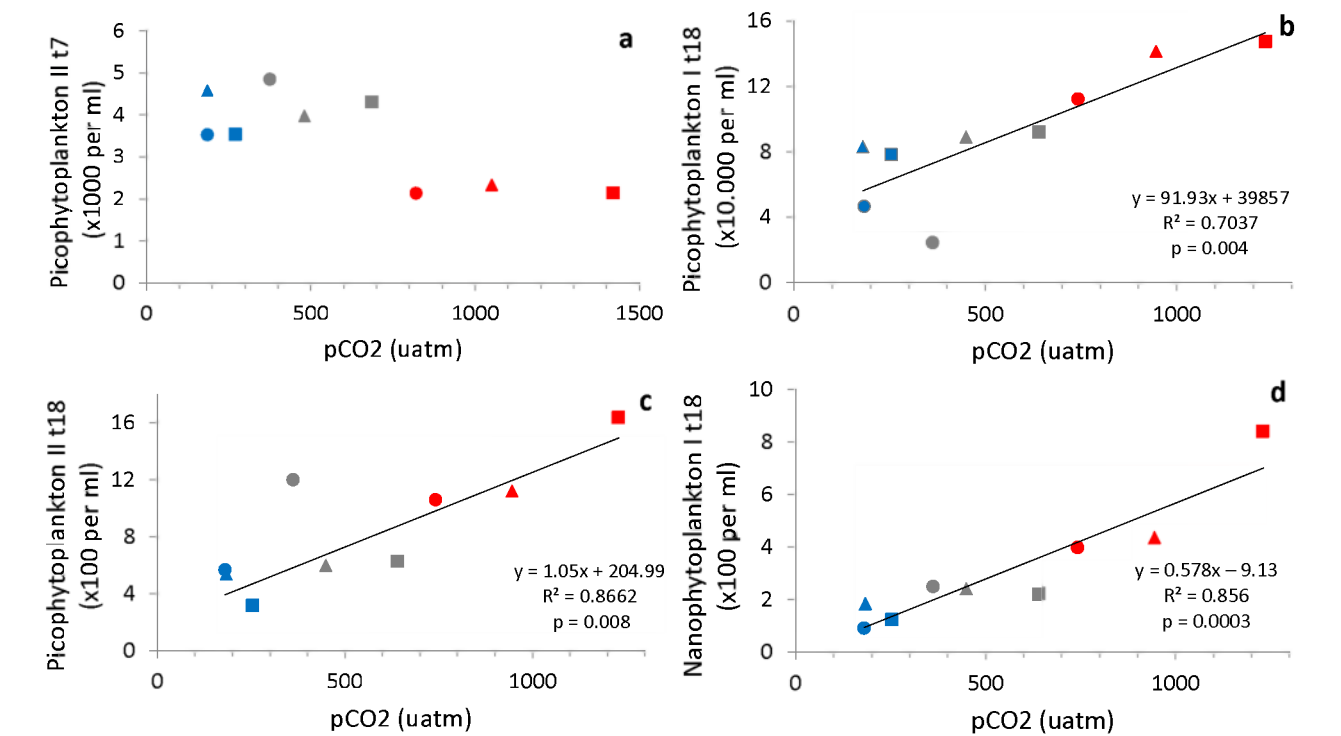
Fig. 3. Phytoplankton cell abundance versus actual p\text{CO}_2 for picophytoplankton II on t7 (a), picophytoplankton I on t18 (b), picophytoplankton II on t18 (c), and nanophytoplankton I on t18 (d). For (b–d) the \text{CO}_2 concentrations plotted were the averages of t8 to t18 . For color and symbol coding, see Fig. 1. Linear regression statistics provided in plots.
