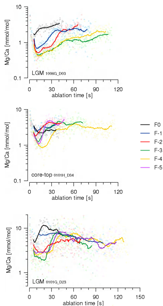
Fig. 6. Mg/Ca profiles through individual N. dutertrei chambers from SE South African margin sediments, both core-top and LGM age. Dots represent raw data, thick lines 25-point smoothed averages that highlight the double-layered structure of the test walls. Note differences in the scale of the y-axes. The difference between the layers is statistically robust at the 95 % confidence interval (Student's t-test on means).
