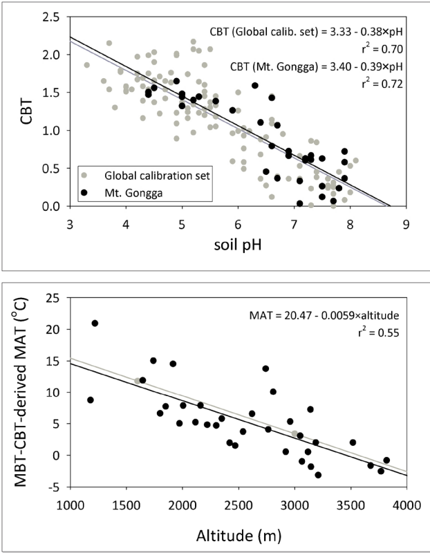
Fig. 4.3. Cross plot of the CBT index vs. measured soil pH for the soils along the eastern slope of Mt. Gongga (black) and for the global soil calibration set of Weijers et al. (2007c) (grey).
