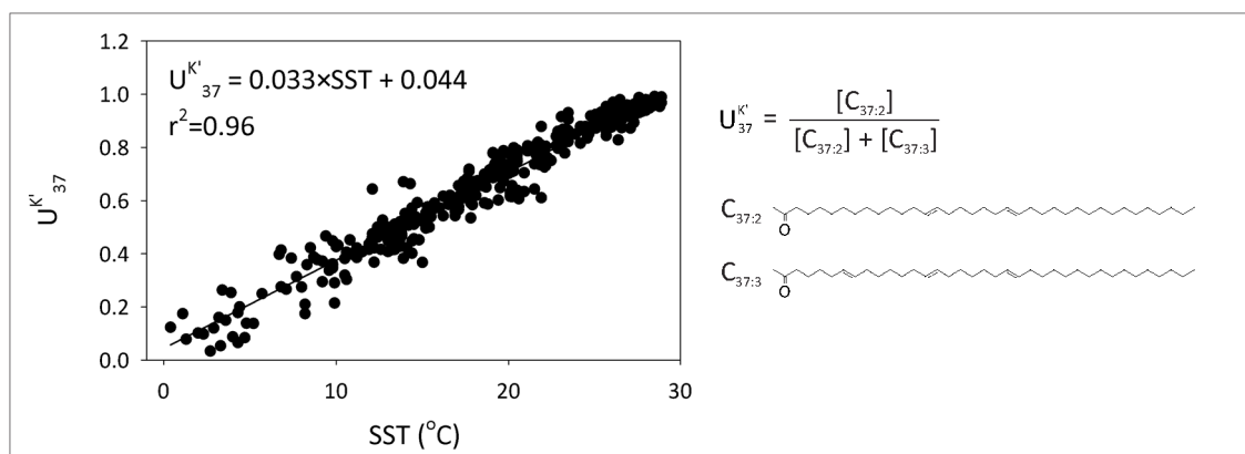
Fig. 1.1. Definition and molecular structures of the alkenones used for the U'_{37} ratio and the relationship between U'_{37} and annual mean SST for surface sediments from the global ocean between 60°S and 60°N (Müller and Fischer, 2004).
