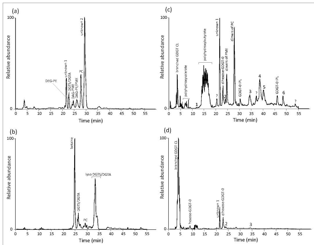
Fig. 7.2. HPLC/ESI-MS base peak chromatograms for the Bligh and Dyer extracts of a) the Saxnäs Mosse peat at 30 cm depth and b) Sphagnum magellanicum , both scanned with an analytical window of m/z 400-2000, c) the Saxnäs Mosse peat at 30 cm scanned with an analytical window of m/z 1000-2000, and d) scanned at m/z after base hydrolysis.
