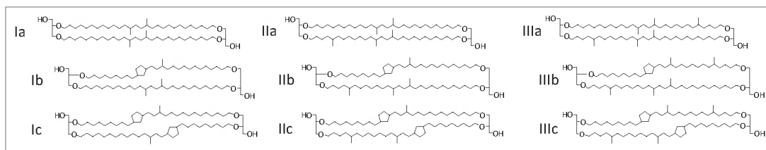
Fig. 8.1. Molecular structures of branched GDGTs.
