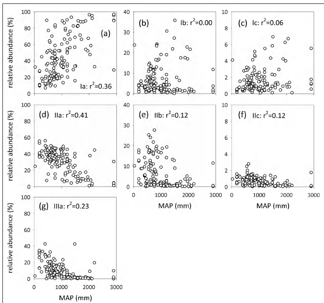
Fig. 8.7. Plots of the relative abundance of each individual branched GDGT (as a percentage of the sum of the seven selected branched GDGTs) versus MAP; a) Ia, b) Ib, c) Ic, d) IIa, e) IIb, f) IIc, g) IIIa. Determination coefficients indicate those of a linear regression.
