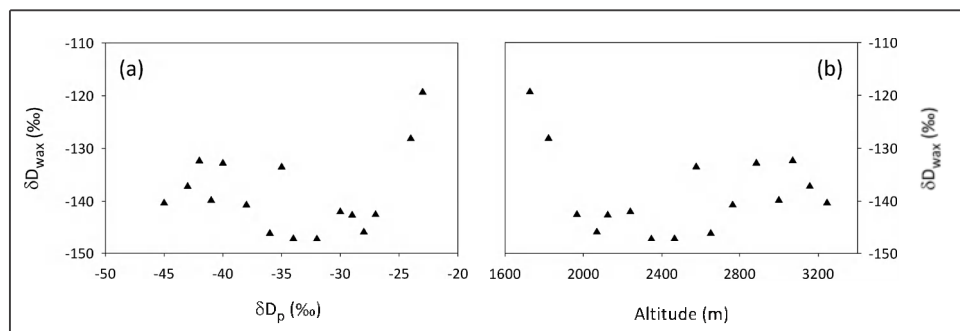
Fig. 4.2. Relations of \delta\text{D}_{\text{wax}} with a) modeled \delta\text{D}_p and b) altitude in ‰ versus VSMOW along the southeastern slope of Mt. Kilimanjaro.
