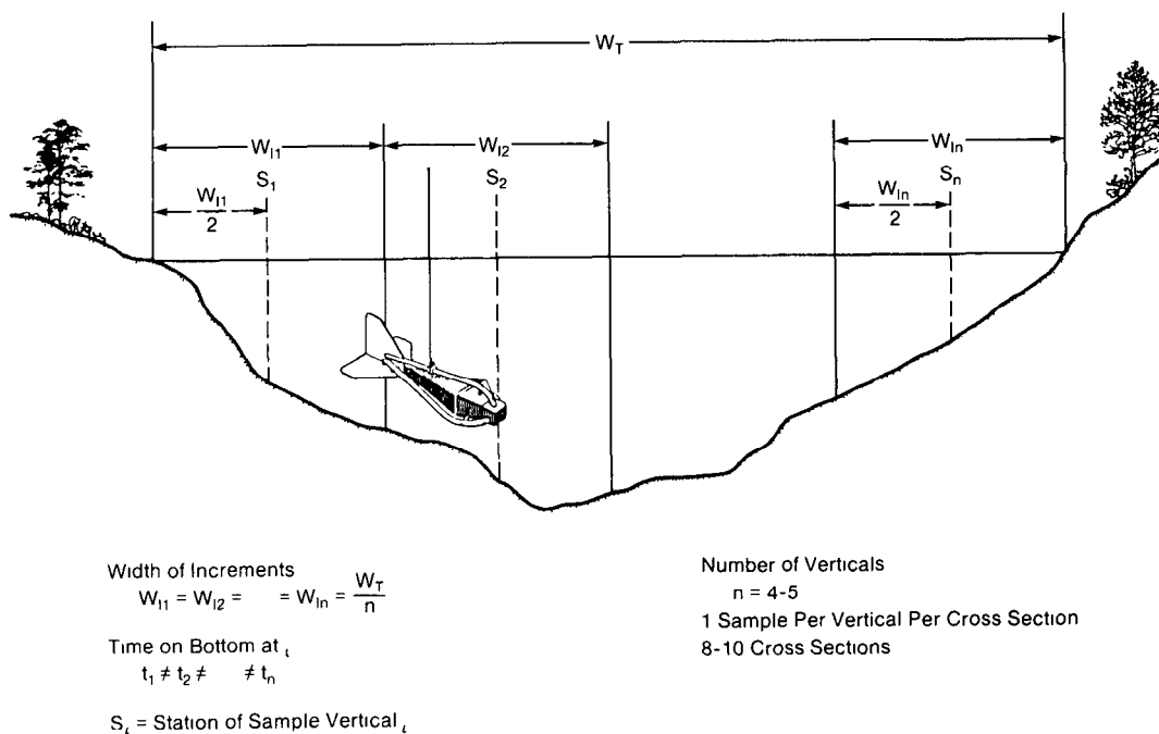
Figure 51. Multiple equal-width-increment bedload-sampling method.
