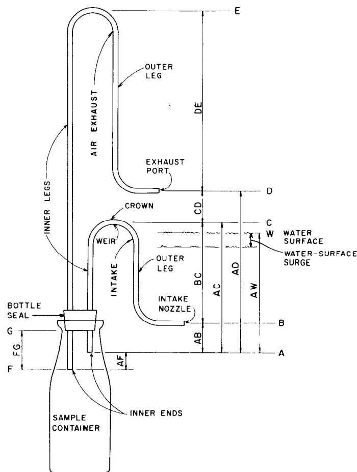
Figure 13. US U-59 single-stage suspended-sediment sampler. Sampling operation using designated letters is described in text (see also Federal Inter-Agency Sedimentation Project, 1961).
