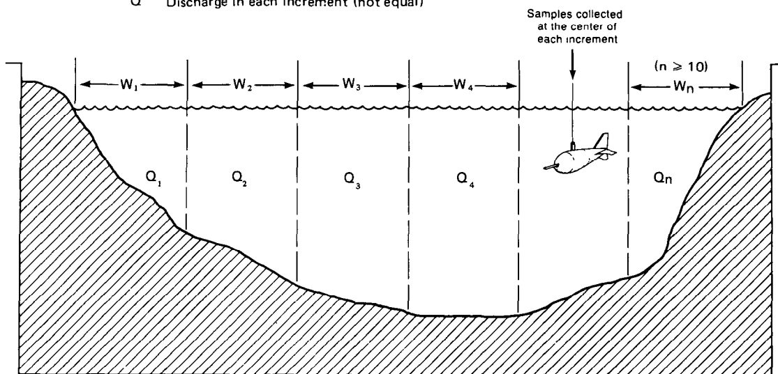
Figure 36. Equal-width-increment sampling technique.
