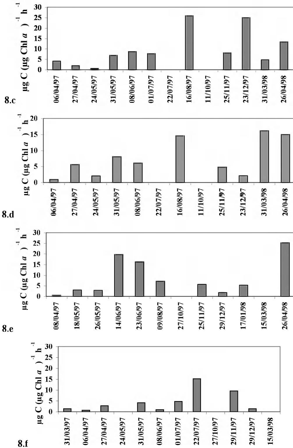
Figure 8. Seasonal distribution of carbon assimilation [ \mu\text{g C } (\mu\text{g Chl-}a)^{-1} \text{ h}^{-1} ] at stations a. K10, b. K6, c. A, d. B, e. 6, and f. 3.
