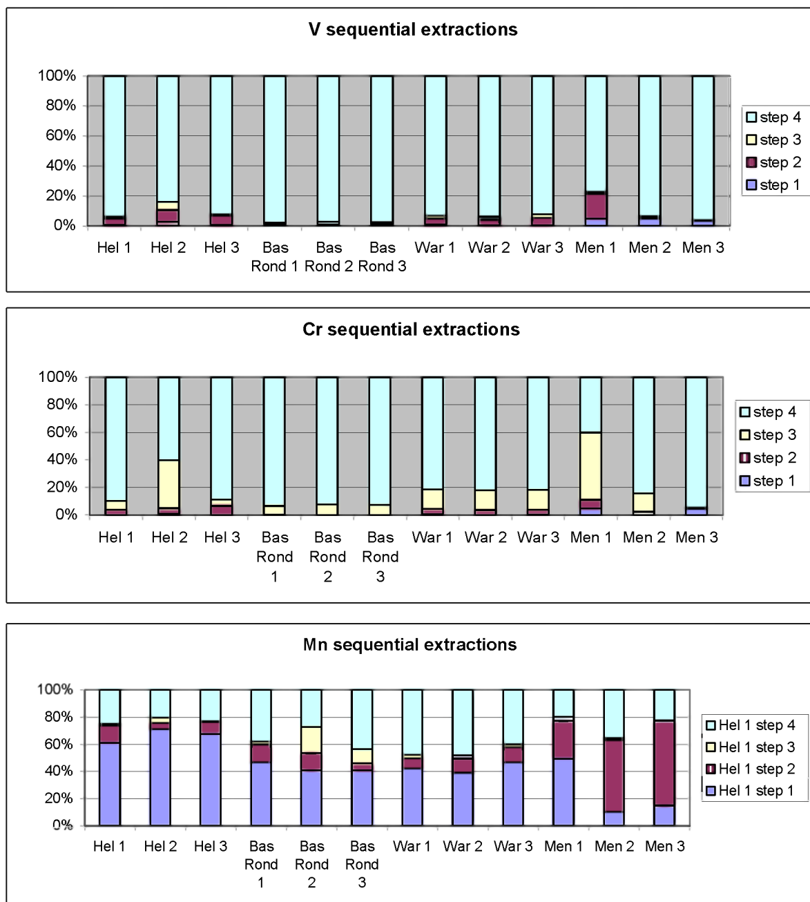
Figure/Figuur 7.18: Trace metal distributions in the different fractions of the sequential extraction technique (at each station 1= 0-2cm; 2= 6-8cm; 3= 16-18cm); step 1: dissolved and exchangeable fraction; step 2: reducible fraction; step 3: oxidizable fraction; step 4: residual fraction
