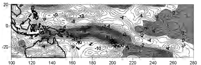
Fig. 2c. The zonal component of the wind velocity (m/s), 04 February 1998 (the third variant of the localization of equatorial westerly winds above the tropical Pacific during the active class), H850.
