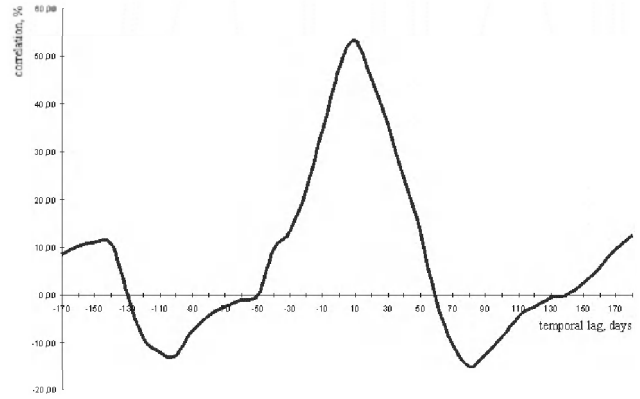
Fig. 4a. Lag-cross correlation function for the temporal coefficients of the first SVD vector: \tau —temporal lag; \tau < 0 : the SST anomalies lag wind anomalies; \tau > 0 : the SST anomalies lead wind anomalies (ENSO 1997–2000).
