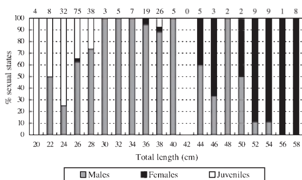
FIG. 4. – Frequency of different sexual states of gilthead seabream in Mellah lagoon as a function of total length. 265 Samples were collected in the months of November and December (see values above).
