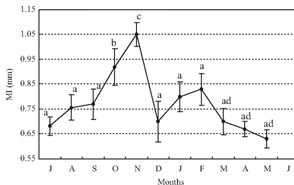
FIG. 1. – Monthly evolution of the marginal increment ( MI = (R_n - R_{n-1}) / (R_n - R_{n-1}) , where R_n and R_{n-1} are the radius of the last and the next-to-last growth rings respectively) of scales of gilthead seabream in Mellah lagoon, Algeria. The different letters indicate significant differences between sampling points.
