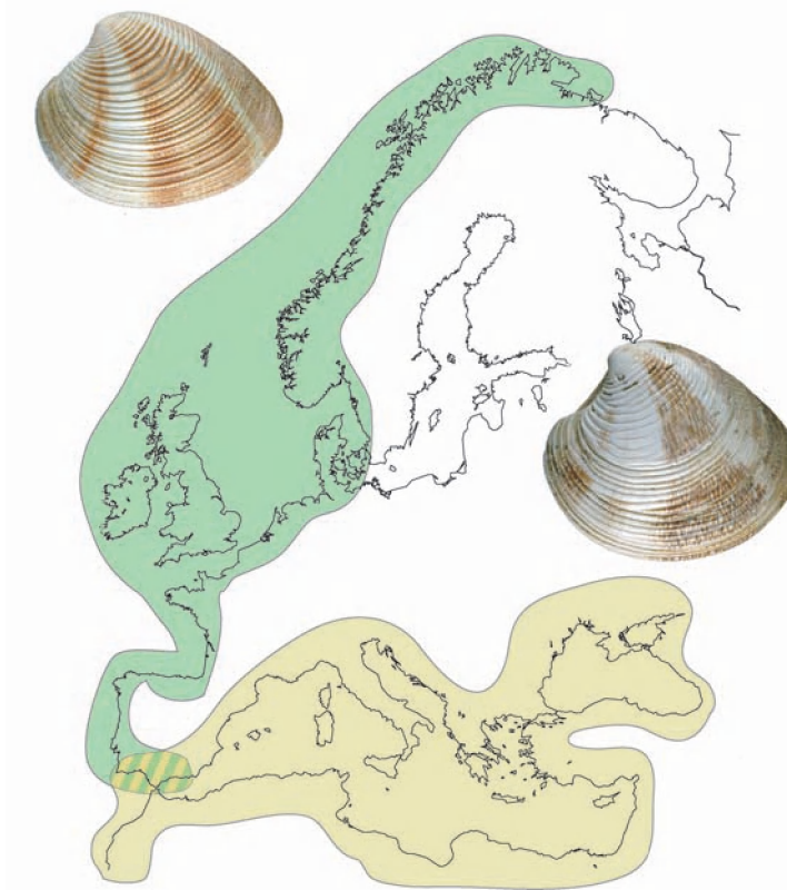
Map 2.1: Distribution of the “Atlantic form” and “Mediterranean form” of Chamelea clams
