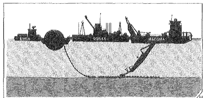
G. Gravel ballast mattress H. The Macoma, the Donax I and the Sepia linked to lay a gravel ballast mattress
