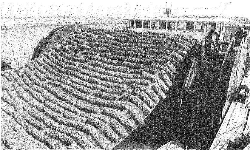
F. Block mattress factory 1 drum 2 concrete blocks 3 rolling track 4 crane for transporting end beams
