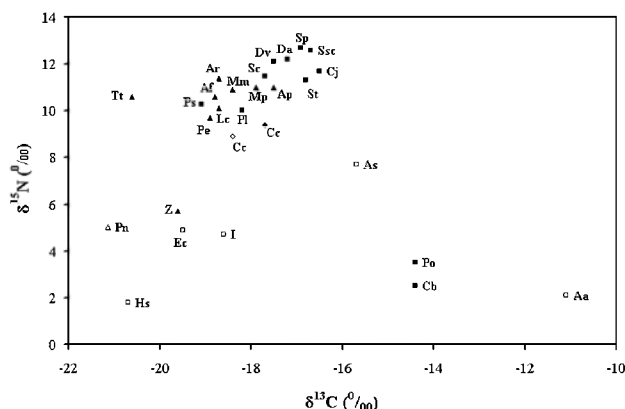
FIG. 2. — \delta^{13}\text{C} and \delta^{15}\text{N} of several species: (○) benthic species from Corsica ( Acetabularia acetabulum (Aa), Halopteris scoparia (Hs), Ircinia sp. (I), Anemonia sulcata (As), Eunicella cavolinii (Ec) (Lepoint et al. , 2000)), (■) benthic species from the Balearic Islands ( Scyllorhinus canicula (Sc), Pasiphaea sivado (Ps), Parapennaues longirostris (Pl) (Polunin et al. , 2001), Coris julis (Cj), Symphodus tinca (St), Diplodus annularis (Da), Diplodus vulgaris (Dv), Sarpa salpa (Ssa), Scorpaena porcus (Sp), Serranus scriba (Ssc) (Jennings et al. , 1997)), (△) pelagic species from Corsica ( Pelagia noctiluca ), (▲) pelagic species from the Balearic Islands (Zooplankton (Z), Alepocephalus rostratus (Ar), Lampanyctus crocodilus (Lc), Merluccius merluccius (Mm), Micromesistius poutassou (Mp), Trachurus trachurus (Tt), Aristeomorpha foliacea (Af), Plesionika edwardsi (Pe) (Polunin et al. , 2001) and loggerhead sea turtles caught in trammel (◆) nets and in long-lines (◇).
