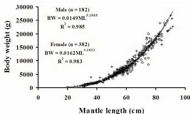
FIG. 2. – Length-weight relationship, by sex, of D. gigas (crosses = male, circle = female).
