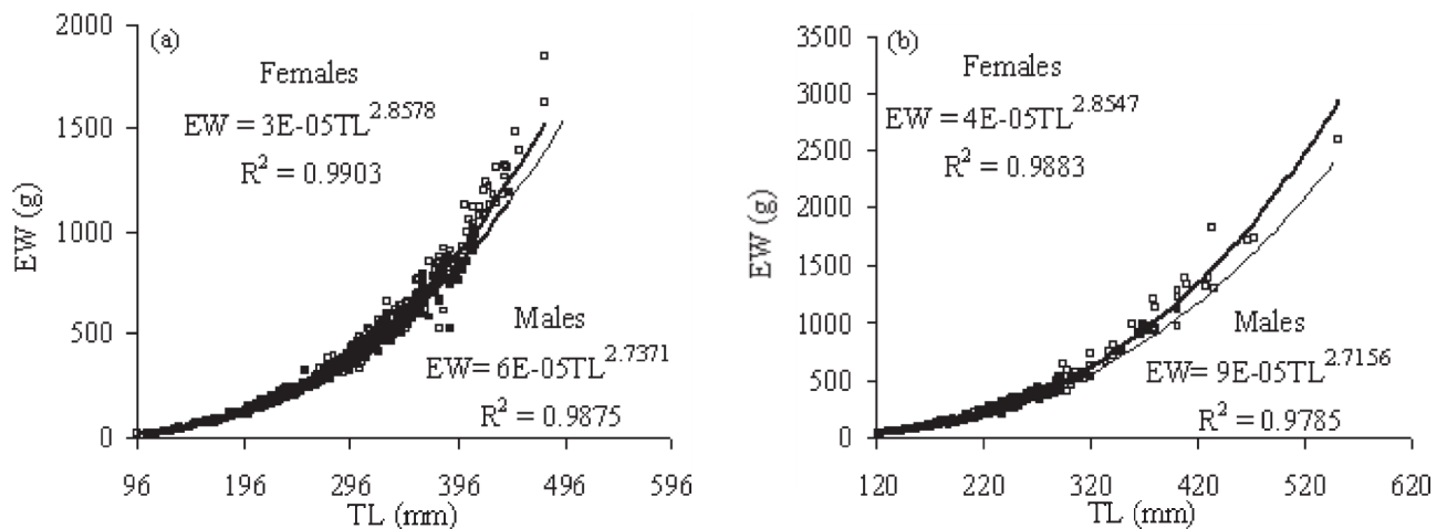
FIG. 3. – Relationships between eviscerated weight and total length in females (□) and males (■) of T. torpedo (a) and T. marmorata (b).
