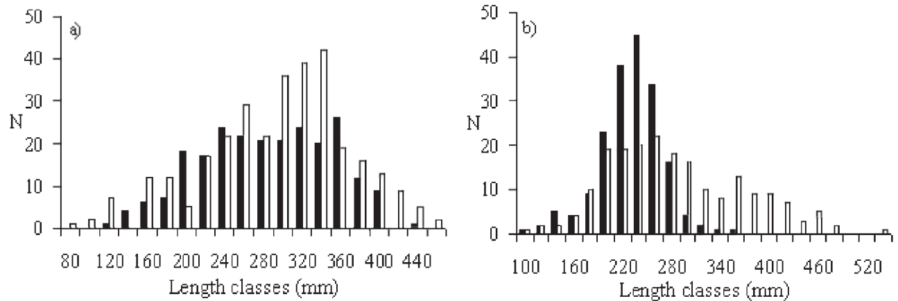
FIG. 2. – Size-frequency distribution by sex (□, females and ■, males) computed by 20 mm width length classes in T. torpedo (a) and T. marmorata (b).
