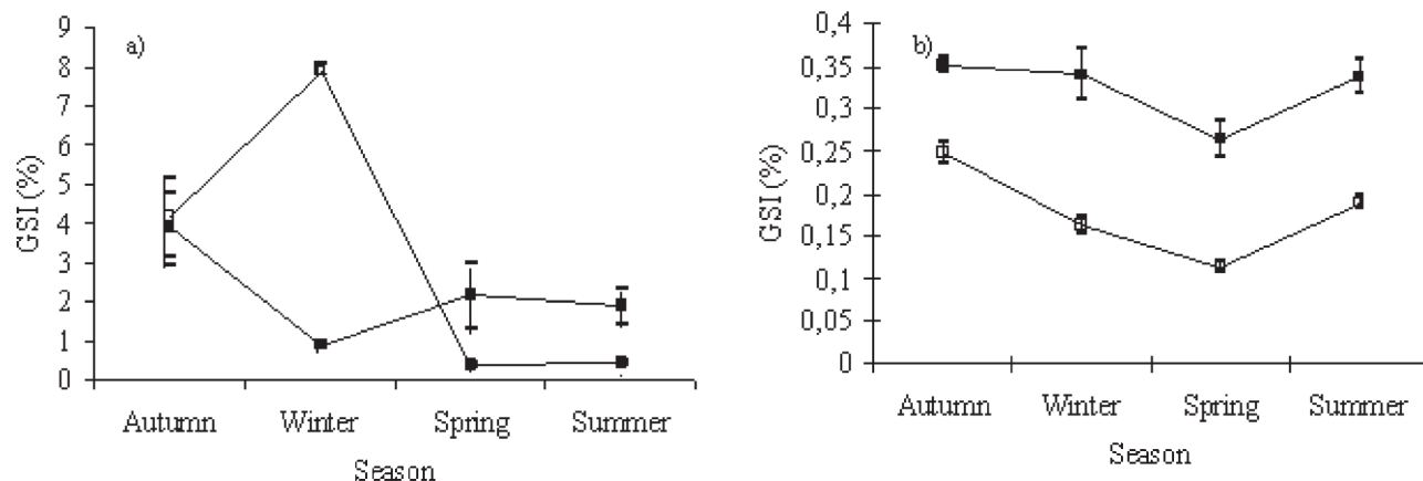
FIG. 4. – Seasonal variation of mean ( \pm S.E) gonadosomatic index (GSI) in females (a) and males (b) of T. torpedo (□) and T. marmorata (■).
