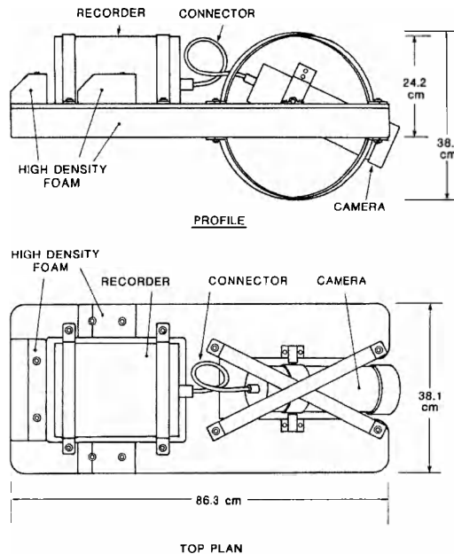
FIGURE 2.—University of Rhode Island underwater camera system composed of a Photosca silicon intensifier target (SIT) camera and Photosca in situ recorder. The unit has the capability to record up to 2 h of data at depths up to 1,000 m (Milliken et al. 1992).
