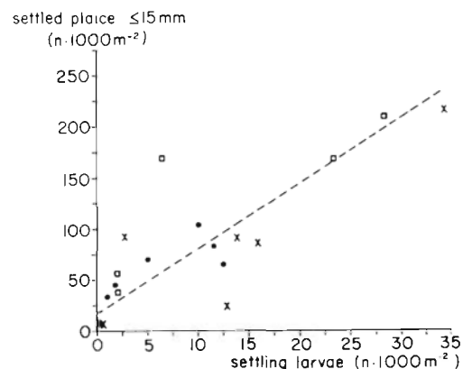
Fig. 10. Pleuronectes platessa . Weekly number of settling plaice larvae (ind 1000m -2 ) per tide estimated from plankton data against simultaneous observed abundances of demersal settled plaice \leq 15 mm. (●) 1980; (x) 1981, (□) 1982
