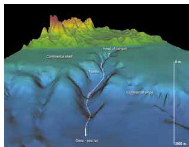
Fig. 6. Topography of a submarine canyon.
