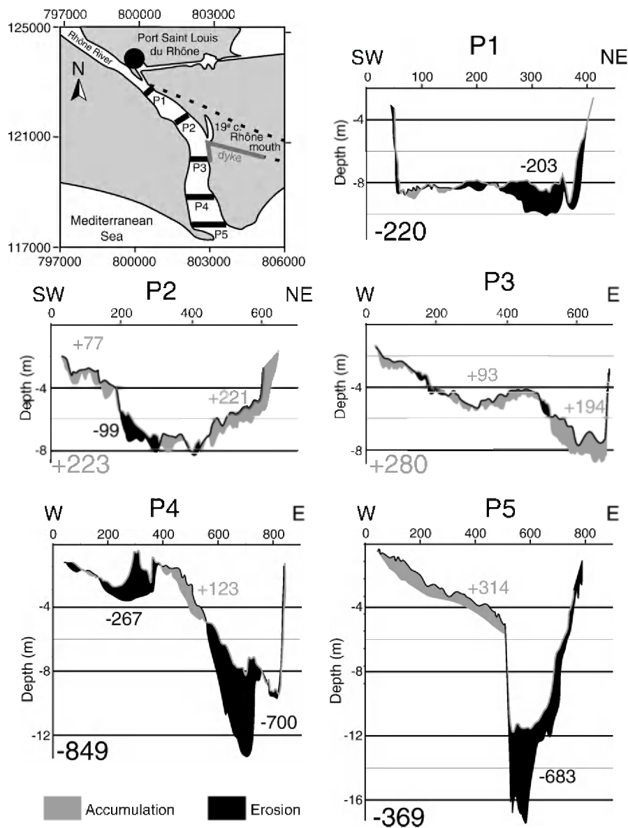
Fig. 8. Overlay of surveyed river-channel sections showing river bed adjustments (in cubic metres) during the 2003 flood event (location of profiles on Fig. 1). Small lettering indicates partial sedimentary budget. Large lettering indicates total budget along each profile. Black and grey figures refer to erosion and accumulation budgets, respectively. To a first approximation, 600,000 m 3 of sediment has been eroded. Maximum sub-channel incision (6 m) occurs in the eastern and lower part of the Rhone River Channel.
