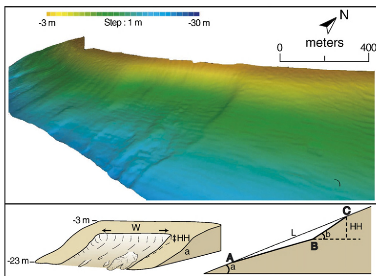
Fig. 5. Morphology of the delta front slope. Sketch detailing the slide area dimensions with: ( W ) is the wide scar, ( L ) is the length scar, ( HH ) is the headscarp height, ( \beta ) is the maximum slope gradient ( 15^\circ ) and ( \alpha ) is the approximate average slope of the delta front (see the text).
