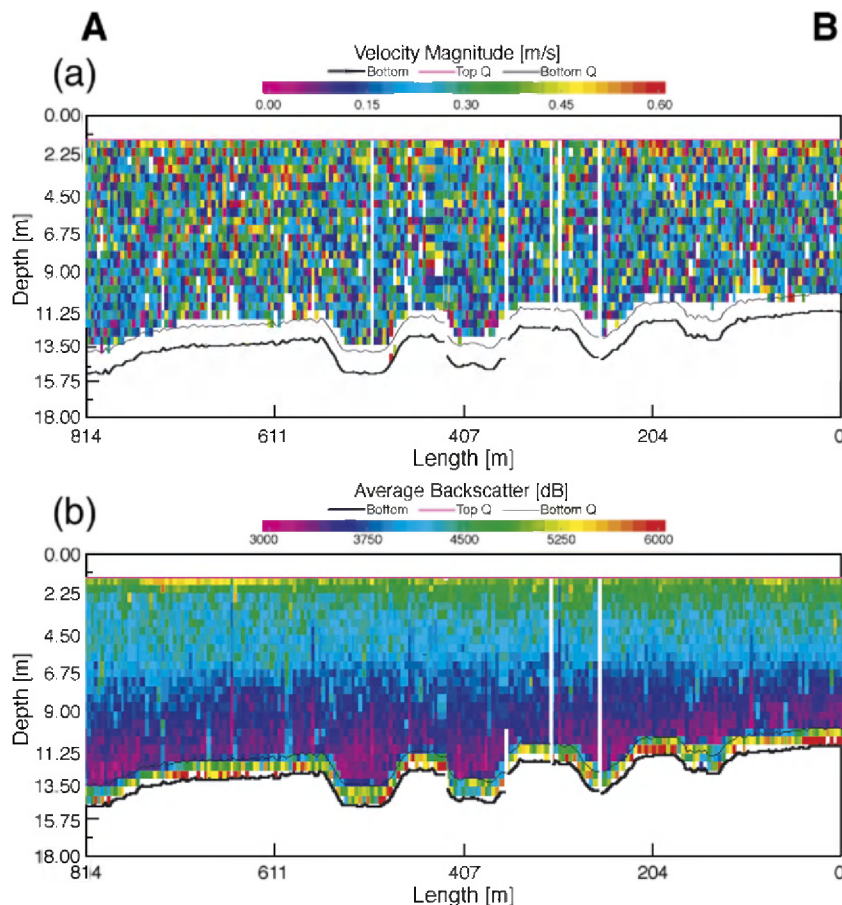
Fig. 7. Hydrodynamic conditions on the delta front slope during low stage period in 2003 November (mean Rhône discharge = 1200 \text{ m}^3 \text{ s}^{-1} , mean wave height = 0.2 m) along AB profile (position on Fig. 1). (a) ADCP-measured current velocity ( \text{m s}^{-1} ) and (b) acoustic backscatter (dB). Backscatter is an indication of suspended sediments in the water column. These images depict homogeneous velocities in the water column with an increase in suspended sediment near the sea surface (plume). Gullies appear to be inactive.
