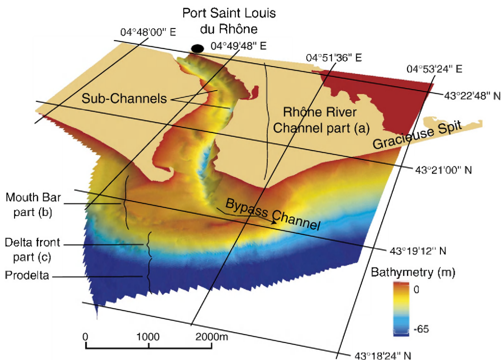
Fig. 3. Bathymetric DTM before 2003 flood event. The study area is divided into three parts: (a) River channel, (b) mouth-bar and (c) Delta front (Rhône03 cruise). In the mouth-bar area, the incised sub-channel is well marked and leads to a shoal mouth-bar. Most of the alluvial flow takes place via a bypass channel through the mouth-bar to the east, and via a broad depressed zone to the west. A slump scar is visible on the delta front, linked to a submarine slide occurring before the December 2003 flood. Submarine gullies on the delta front slope extend from the base of the mouth-bar to the top of the prodelta (between -4 \text{ m} and -30 \text{ m} isobaths).
