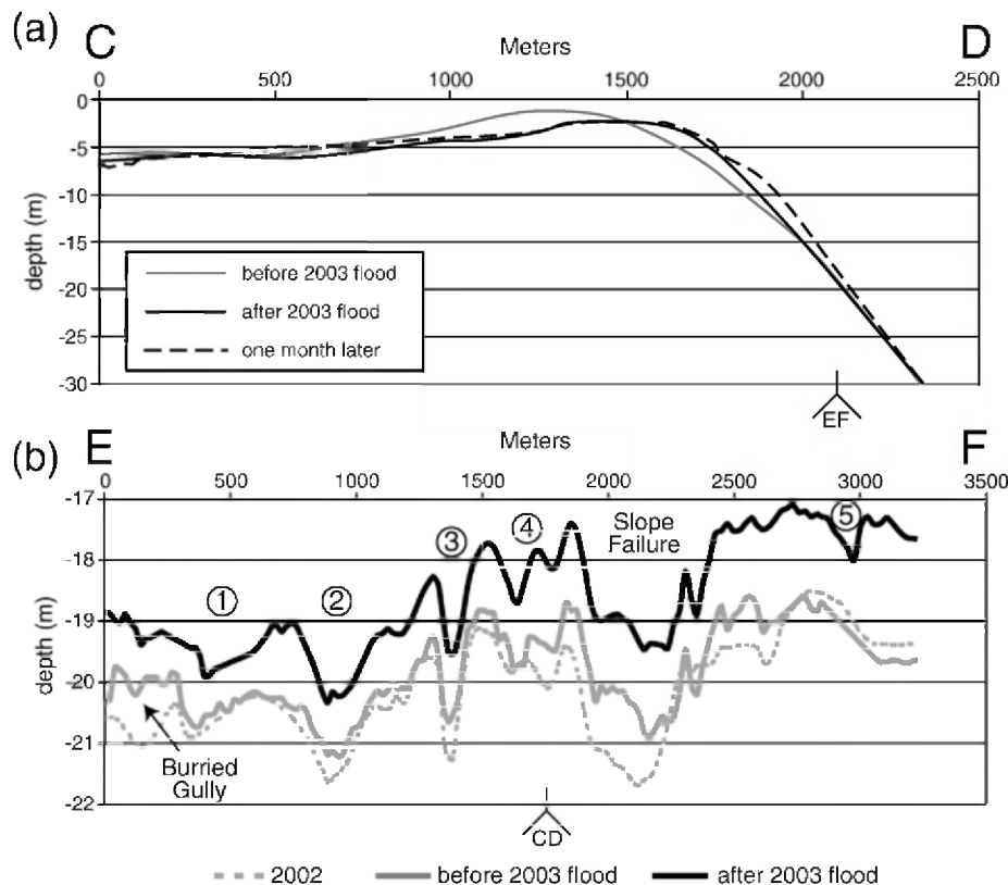
Fig. 10. Bathymetric variation along two profiles across the Rhône subaqueous lobe from DTM data. Detailed location on Fig. 1 (a) cross-shore profiles before the 2003 flood event (Rhône03 cruise), just after flood event (MATRhône1 cruise) and one month later (MATRhône2 cruise). Post-flood deposition mechanisms are highlighted and sediment remobilisation by waves is in evidence down to 6 m depth. (b) long-shore profiles across the delta front. The 2002 profile (Strataform1 cruise) is used as a reference profile. Bathymetric and morphological changes induced by the 2003 flood event are shown comparing the pre-flood and post-flood profiles. Numerals define the order of gullies in an eastward direction. Features are preserved during the flood event, so settling out processes are presumed predominant. Note the creation of a new channel during the flood event (n°5), being the morphological expression of local hyperpycnal coarse sediment transfer.
