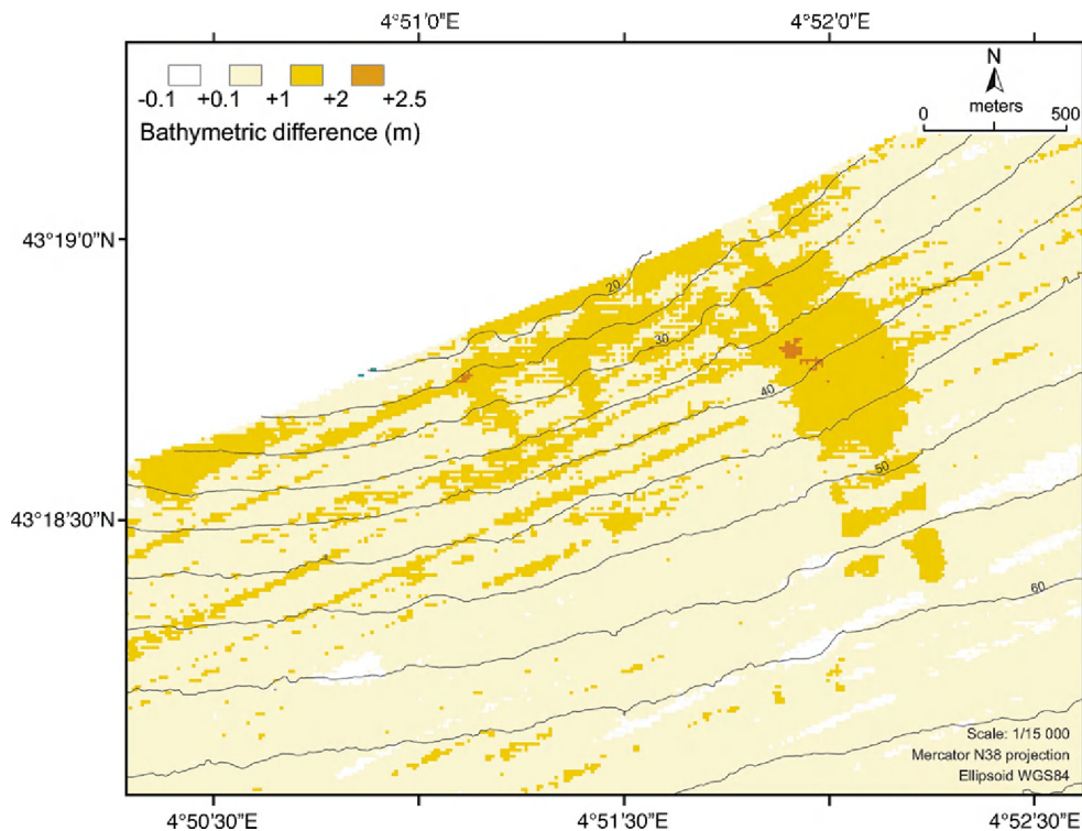
Fig. 6. Morpho-bathymetric difference observed between the multibeam surveys of May 2002 and December 2003 (Cruise Strataform1 and RhoneFlood) on the prodelta area. Only a thin cover of sediment was deposited in this zone since 2002 and slide mass shape was not deleted by 2003 flood event dynamics.
