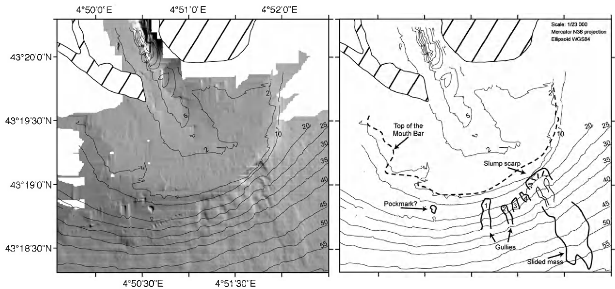
Fig. 4. Detailed bathymetric DTM of the Grand Rhône subaqueous lobe with evidences of slope failure and gullies.
