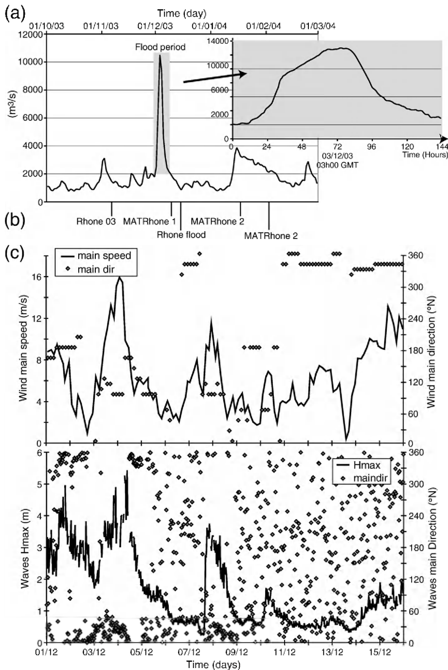
Fig. 2. Flood hydrographs at Beaucaire gauging station for 2003 flood event: (a) Mean daily liquid discharge ( \text{m}^3 \text{s}^{-1} ) and mean hourly liquid discharge ( \text{m}^3 \text{s}^{-1} ). (b) Timing of cruises. (c) Climatic conditions during the flood period. Directions are designed with conventional marine chart (origin direction for wind and displacement direction for waves).
