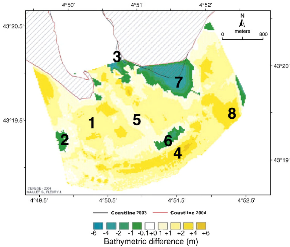
Fig. 9. Bathymetric changes in metres during the 2003 flood event at the Rhône mouth, between 0 and -20 m depth. A significant total volume ( V_t ) of 7.8 million \text{m}^3 (about 4 million tons) was sedimented in this area, corresponding to a mean volume per unit area ( V_m ) of about 0.88 \text{ m}^3 \text{ m}^{-2} . These values are in accordance with upstream fluvial measurements that quantified flood solid discharge between 3.1 and 5.28 million tons.
