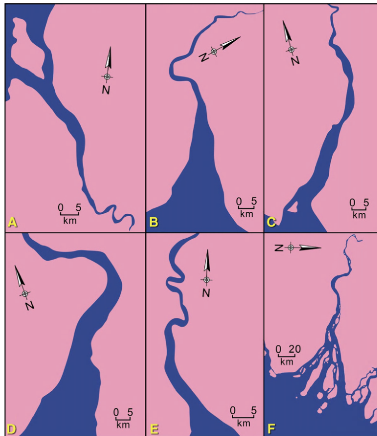
Fig. 21. Six examples of coastal systems that display a funnel-shaped geometry (i.e., the width increases exponentially with distance seaward): (A) Ord River, Australia; (B) Khor Abdullah, Iraq; (C) Irrawaddy River, Myanmar (Burma); (D) Hoogly River, India; (E) Cua Soirap, Vietnam; (F) Fly River, Papua New Guinea. Note that in most of the systems, the sinuosity of the channel increases as it becomes narrower. (A–E) Modified after Wright et al. (1973) and reproduced with permission of the University of Chicago Press.
