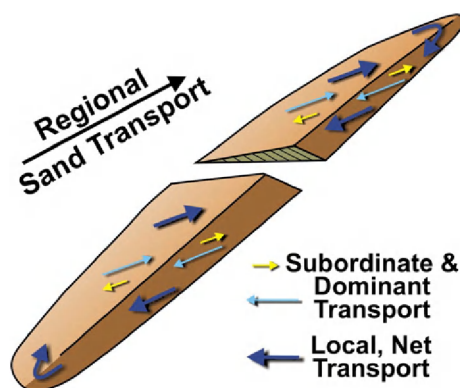
Fig. 29. Schematic diagram illustrating the oblique cross-bar flow over an elongate tidal bar. The resulting migration of the bar is oblique, but predominantly transverse to, the direction of the regionally dominant (stronger) current and to the bar crest. This leads to the preferential preservation of the down-current flank of the bar, where sedimentation is dominated by the subordinate current. As a result, the small cross beds within the large-scale lateral-accretion deposits are likely to be oriented in the direction of the regionally weaker current! After Dalrymple (1992).
