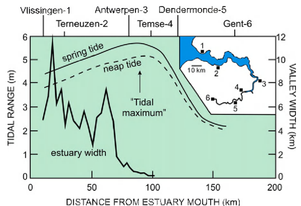
Fig. 5. Longitudinal variation of estuary width and tidal range in the Westerschelde estuary, The Netherlands. Place names (top) keyed to inset map. Note how the tidal range increases landward as the estuary width decreases, reaching a peak range (the “tidal maximum”) inland of Antwerp. Modified after Van der Spek (1997).
