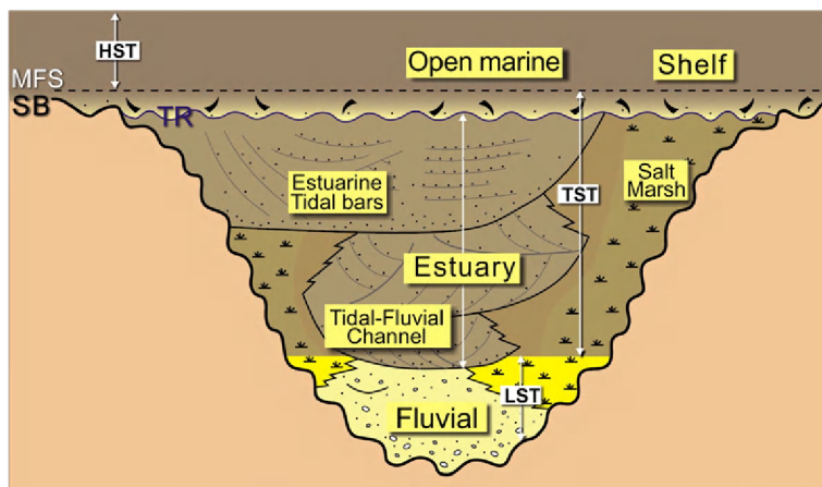
Fig. 6. Schematic vertical cross section of a tide-dominated estuary located within an incised valley (see map view in Fig. 9). The overall succession is transgressive in character, with fluvial deposits at the base, overlain by estuarine deposits, and capped by open-marine deposits of the succeeding progradation. Systems tracts are noted. Within the estuarine deposits, note that the sandy channels become larger (wider) upward, reflecting the seaward-flaring, funnel shape of this type of system (see Figs. 9 and 21 below). These sandy channel deposits are flanked by muddy tidal-flat and salt-marsh sediments. After Dalrymple (1992).
