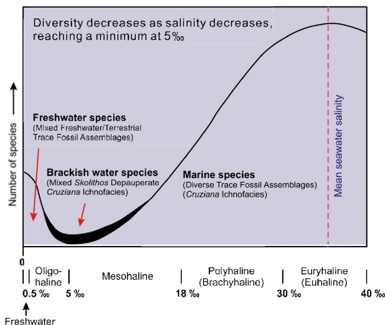
Fig. 20. Classification of salinity levels and variation of species diversity through the freshwater to seawater transition. Note that brackish-water environments have low taxonomic diversity and are characterized by a mixed Skolithos – Cruziana ichnofacies. After Buatois et al. (1997). Courtesy of SEPM (Society for Sedimentary Geology).
