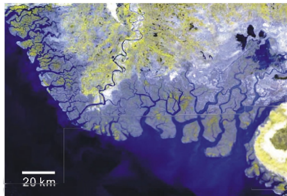
Fig. 1. Satellite image of the Indus River delta ( sensu lato ). The area of active river outflow occurs at the apex of the deltaic protrusion in the centre of the image. Only this part of the coast and the immediately adjacent areas are receiving river-supplied sediment directly from the river; hence, this is the only part of the system that is actively prograding at the present time (i.e., it is the only part of the system that is truly deltaic in the context used in this paper). The remainder of the delta plain is inactive (i.e., abandoned) and is inferred to be undergoing slow transgression due to tectonic subsidence and/or compaction of the underlying mud. Thus, the many sinuous tidal channels in the abandoned part of the larger delta complex behave as estuaries, as defined herein. For more information on this delta, see Brookfield (1998) and Prins et al. (2000). Courtesy of European Space Agency (ESA).
