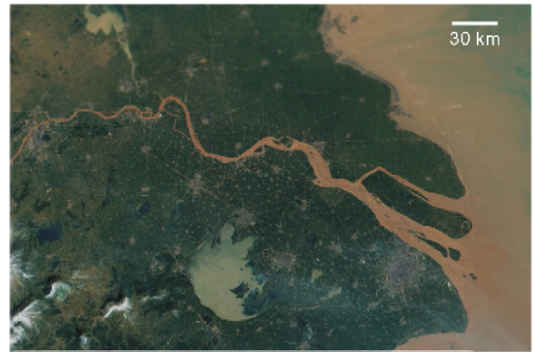
Fig. 24. Satellite image of Yangtze River delta, China (spring tidal range 4.9 m). Note the seaward widening and straightening of the channels, although the funnel shape is less pronounced than in some other systems because of the large river discharge. For more information on this system, see Hori et al. (2002) and Li et al. (2002). Courtesy of NASA.
