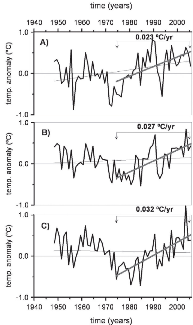
FIG. 12. – Sea surface temperature anomalies from the NCEP. A, Alboran Sea, B, Balearic Sea, and C, Northern Sector. The thick line is the linear trend for the period 1974–2005. The corresponding figure is inserted for comparison with Salat and Pascual (2002, 2006). The thin black line is the linear trend for the period 1950–2005, for comparison with Krahmann and Schott (1998).
