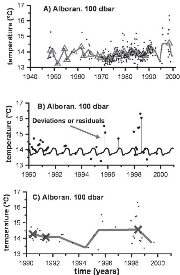
Fig. 3. – Figure 3A illustrates the large noise variance in monthly time series, especially in the upper layers (black dots). The grey line is the time series when the annual seasonal cycle has been filtered out using yearly averages, and open grey triangles show the yearly averaged time series when a restriction is imposed, in this case that valid years should contain data for at least the four seasons of the year. Figure 3B is an example of extraction of the seasonal climatological cycle. Figure 3C is a zoom of Figure 3A and shows the data point reduction when some restrictions are applied to the data validity.
