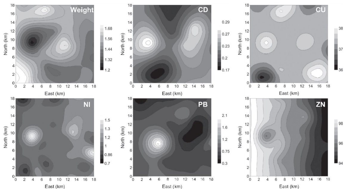
FIG. 4. – Mapped spatial distribution of weight ( mbww = mean body wet weight of shrimps per sample in g), Cd , Cu , Ni , Pb and Zn in Crangon crangon ( mg\ kg^{-1} DW, respectively) within Box A (Fig. 1) in universal kriging plots showing contour lines.
