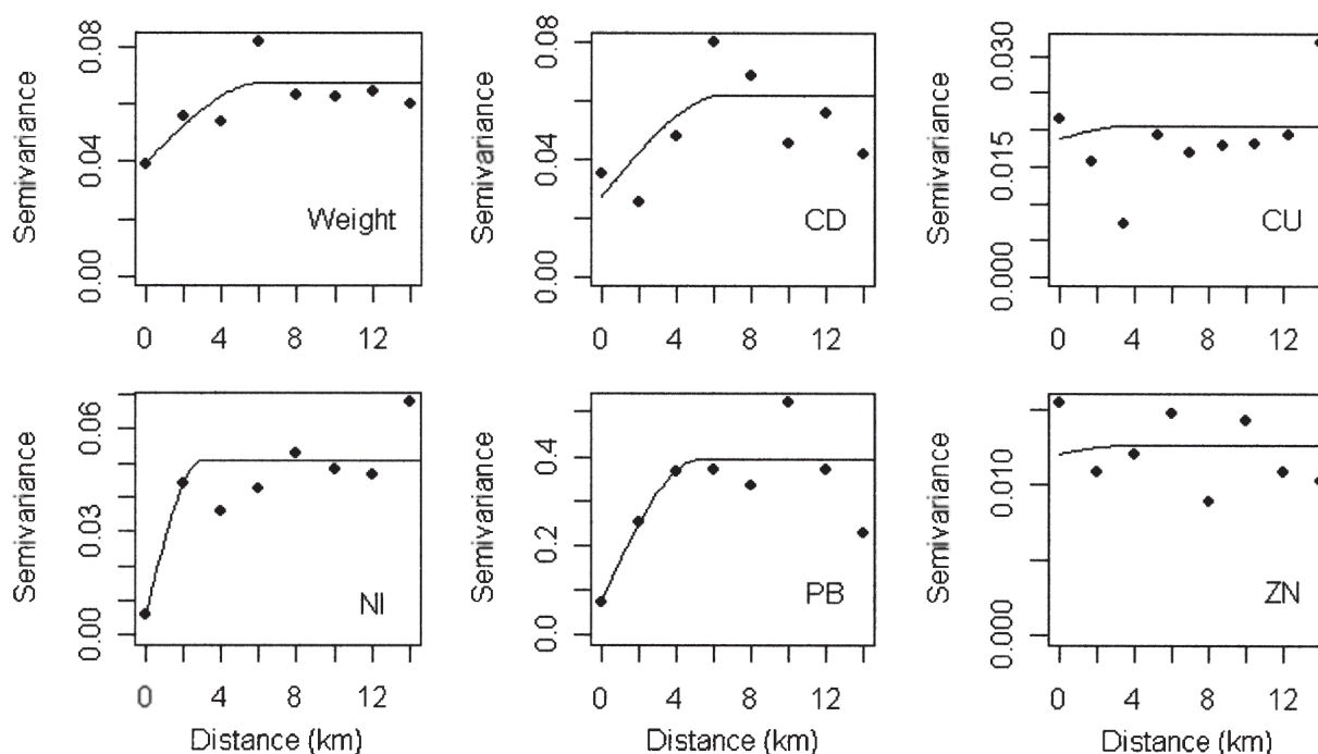
FIG. 3. – Empirical semivariograms with fitted spherical models for weight ( mbww = mean body wet weight of shrimps per sample in g), Cd , Cu , Ni , Pb , and Zn in Crangon crangon ( \text{mg kg}^{-1} DW, respectively) within Box A (Fig. 1).
