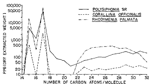
FIG. 1. Normal alkane content of red algae.
