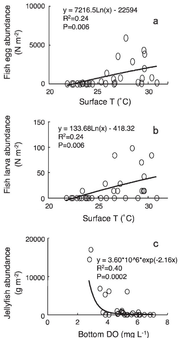
FIG. 4. — Plots of (a) fish egg and (b) fish larval abundance to sea surface temperature (T, °C), and (c) jellyfish abundance to bottom oxygen concentration (DO). Data from the Sea of Hiuchi and Hiroshima Bay are combined.
