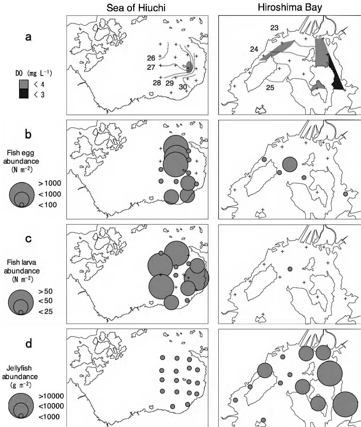
FIG. 3. – Horizontal distribution of sea-surface temperature ( ^{\circ}\text{C} , contours) and (a) bottom oxygen concentration (DO), (b) fish egg, (c) fish larvae and (d) jellyfish abundance in the Sea of Hiuchi and Hiroshima Bay. Crosses indicate sampled stations.
