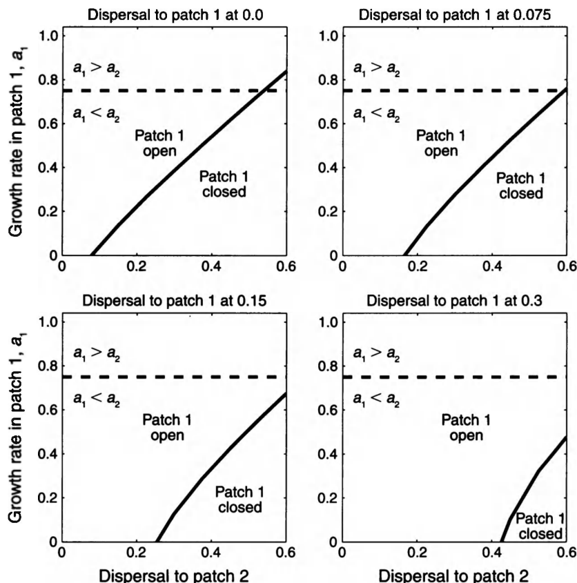
FIG. 8. Density-independent and density-dependent settlement and critical growth rates for different dispersal rates to patch 1. By holding the share of juveniles from patch 1 (reserve designate) fixed at a particular level, we illustrate how the critical growth rate changes as the share of juveniles from patch 1 (reserve designate) to patch 2 (fished area) increases. Costs are equal across the patches. Regions in the panels illustrate the optimal solution whereby, for example, it is optimal to have both patches open to fishing ( a_1 < a_1^{\text{crit}} ) or to close patch 1 to fishing ( a_1 \geq a_1^{\text{crit}} ). The dashed line represents the critical growth rate in patch 2 ( a_2 ). When the critical growth rate (solid line) is above the dashed line, it is optimal to close the high-productivity patch. The upper left panel represents the case of unidirectional flows of juveniles (patch 1 is a source of larvae, and patch 2 is a sink). The other panels represent different levels of larval flows from patch 2 to patch 1. Points to the left of the intercept on the x-axis are infeasible.
