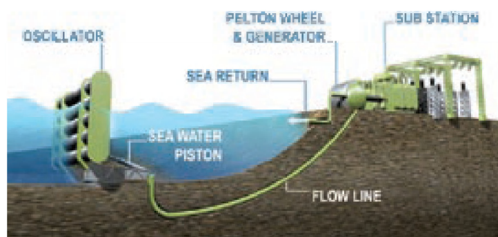
Aquamarine Power Ltd – Oyster wave surge converter
