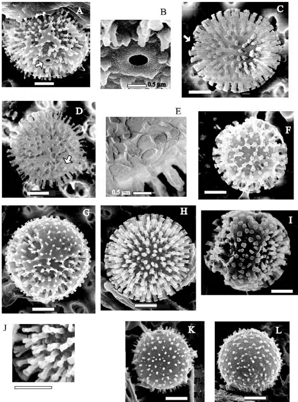
Fig. 4. a–e, g, h & j. Litheusphaerella cf. spectabilis Deflandre form 2. f. & i. L. cf. spectabilis Deflandre form 1. k. & l. Archaeomonas cf. japonica Deflandre. Scale bars = 0.5 μm (b & e), others = 2 μm.
