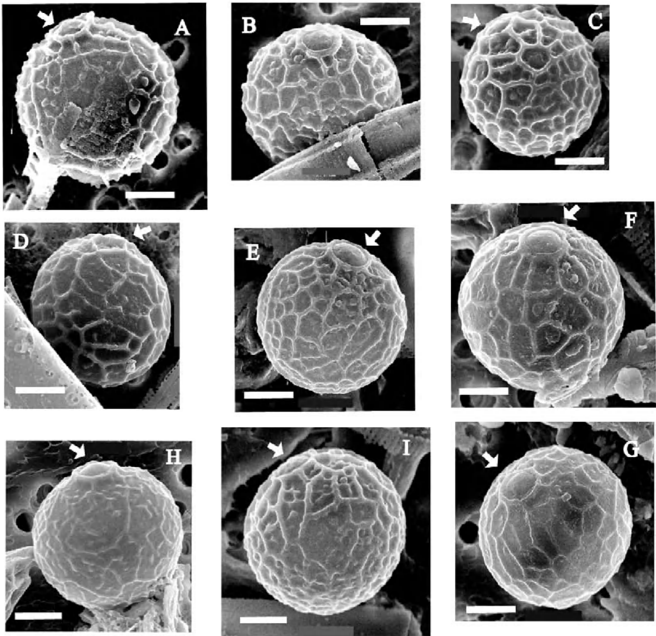
Fig. 3. a–g, Archaeomonas cf. speciosa Deflandre. h, (?) A. cf. helminthophora Deflandre. i, (?) A. cf. auranticutosa sp. nov. (see Fig. 1h). Scale bars = 2 μm.
