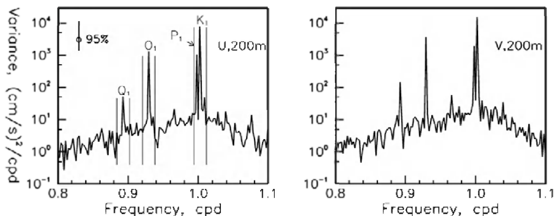
Fig. 2. Diurnal-band spectra of 5 years of mooring B' velocities, showing the major tidal constituents and their 1/(56 \text{ day}) width demodulation bands. 95% confidence limits are shown.
