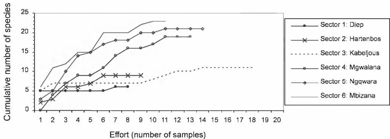
Figure 2. Relationship between sampling effort (seine and gill netting) and number of species captured in representative closed estuaries from each coastal sector.
