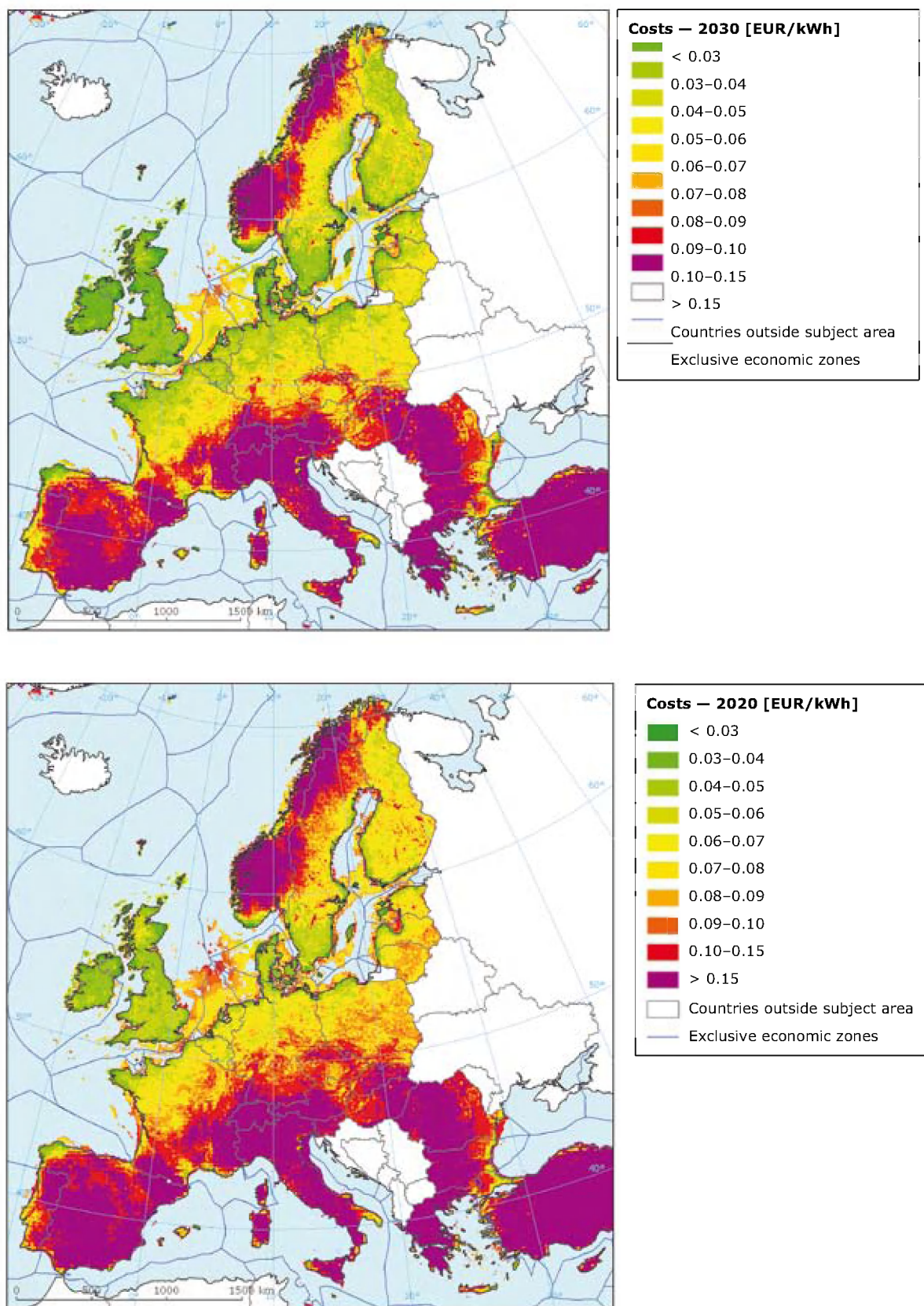
Map 6.3 Generation costs for wind energy in Europe (left 2030, right 2020)
