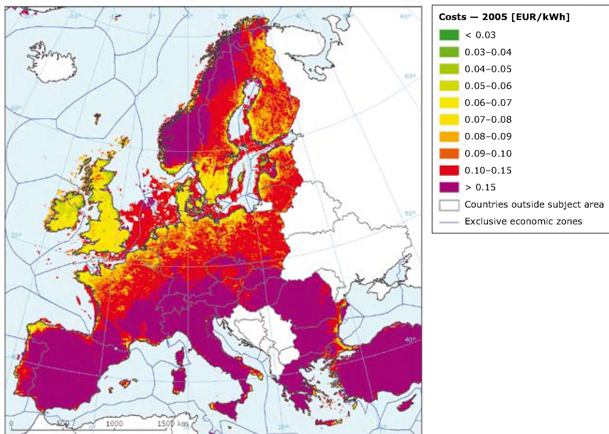
Map 6.2 Generation costs for wind energy in Europe, 2005
