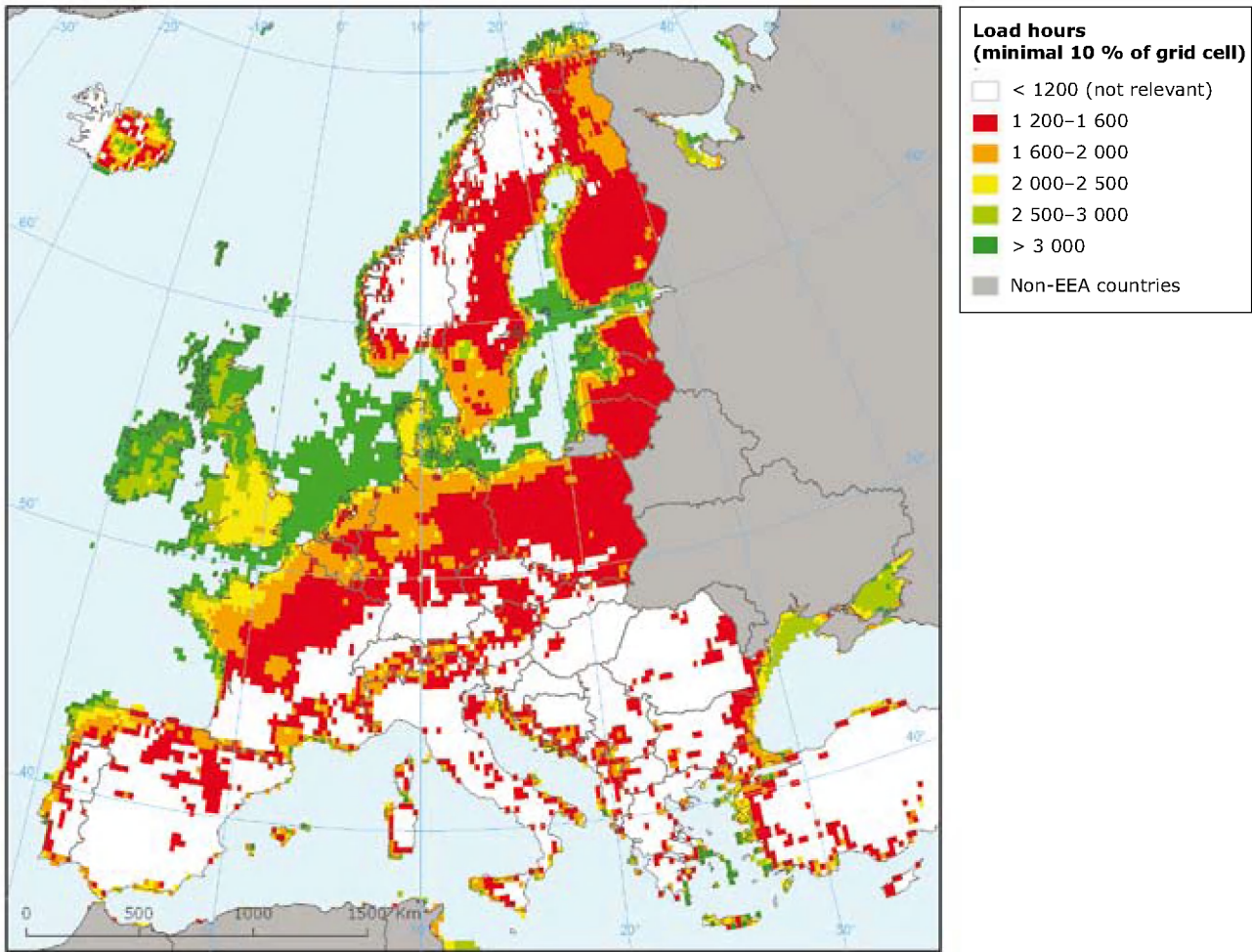
Map A4.1 Distribution of full load hours in Europe for the ninetieth percentile (at least 10 % of the sub grids has the minimal indicated load hour)
