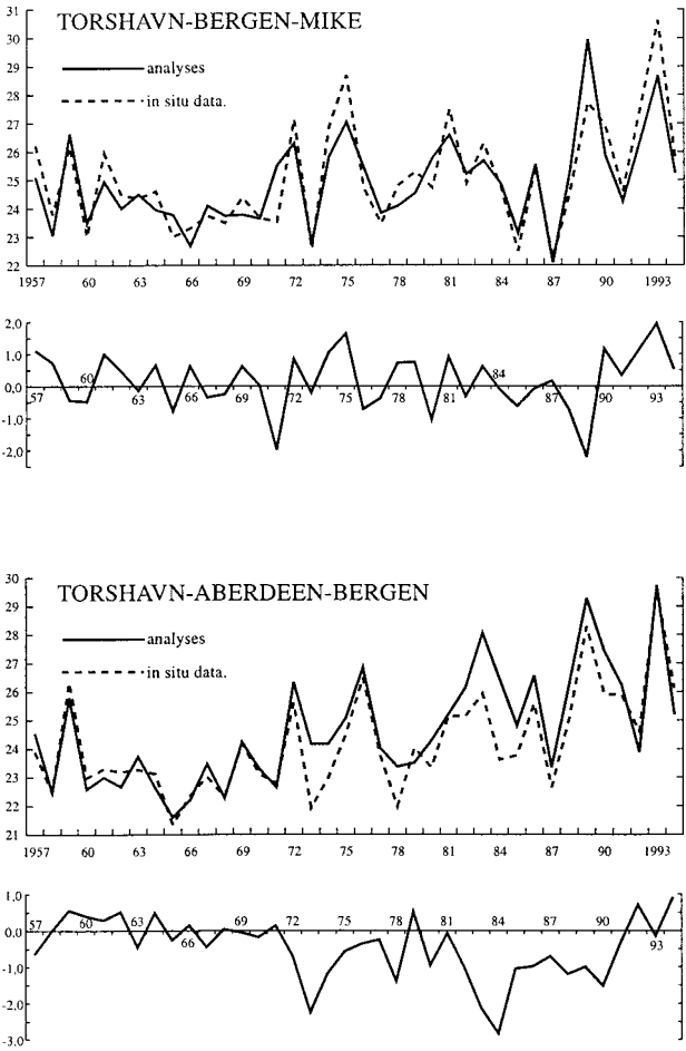
FIG. 8. Time series of annual 90% percentiles of geostrophic wind speeds derived from in situ data (top: Thorshavn–Ocean Weather Station M–Bergen; bottom: Thorshavn–Aberdeen–Bergen) and from the operational DNMI analyses. In the lower panels, the difference between the two curves in the upper panels is given. Units: \text{m s}^{-1} .
